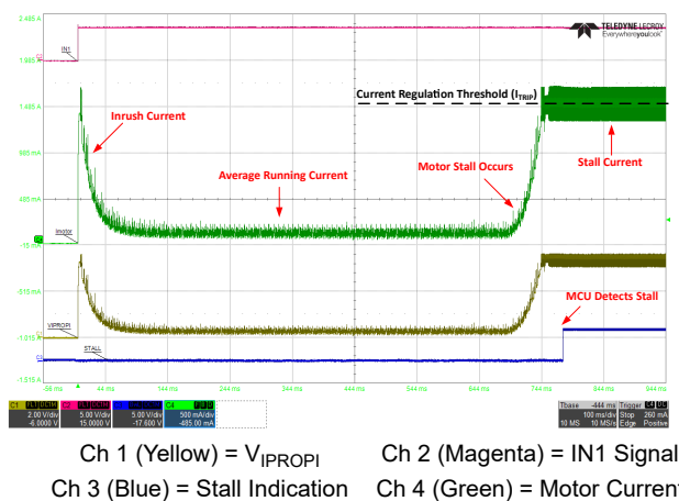
图 9-7. Example Waveform of Stall Detection
