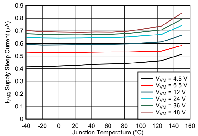
图 7-2. Sleep Current ( I_{VMQ} ) vs. Junction Temperature ( T_J )
