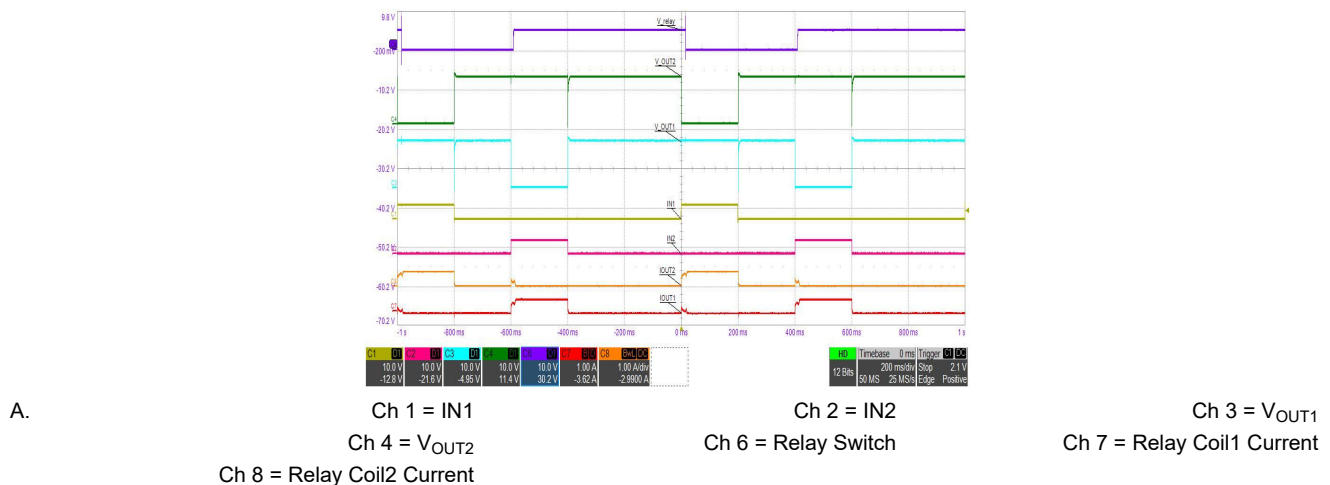
图 9-15. PWM driving for dual-coil relay
