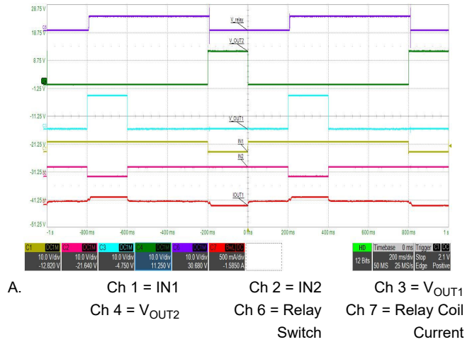
图 9-14. PWM driving for a single-coil latching relay with driving profile FORWARD → BRAKE → REVERSE → BRAKE
