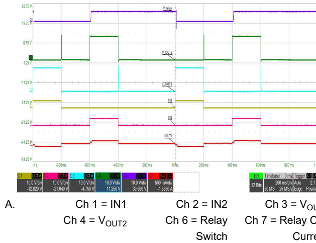
图 9-13. PWM driving for a single-coil latching relay with driving profile FORWARD → COAST → REVERSE → COAST
