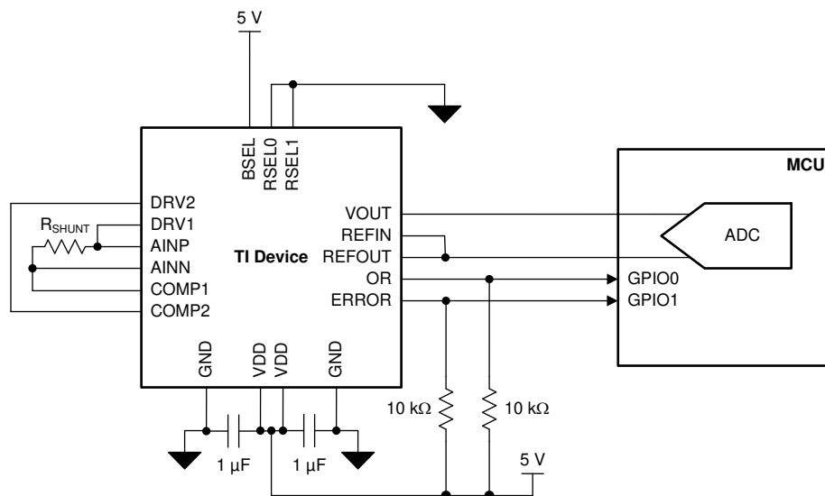
图 67. Linear-Position Sensing
