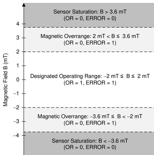
图 63. Magnetic Field Range of the DRV425-Q1 (VDD = 5 V and R_{SHUNT} = 22\ \Omega )
