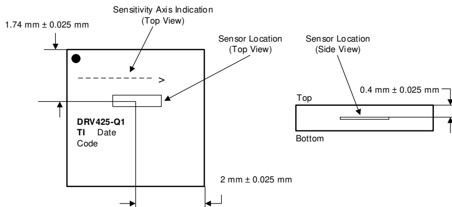
图 61. Magnetic Sensitivity Direction of the Integrated Fluxgate Sensor
