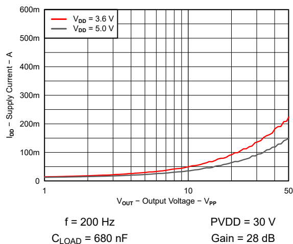
图 6-7. Supply Current vs Output Voltage
