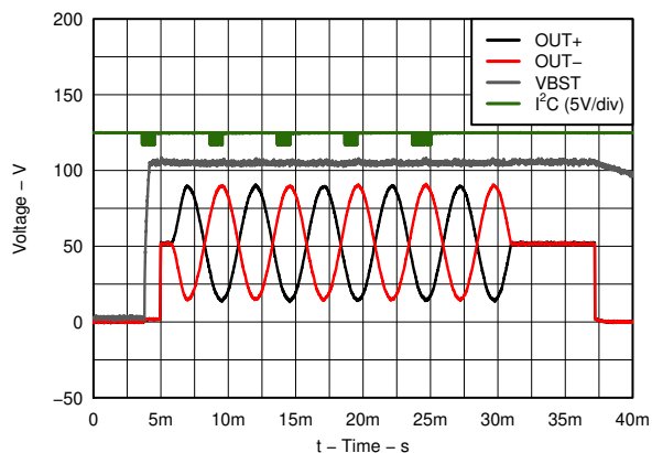
图 6-10. Typical Waveform
