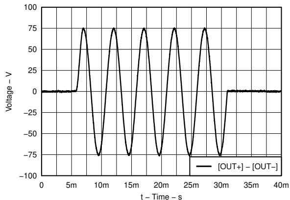
图 6-10. Typical Waveform
