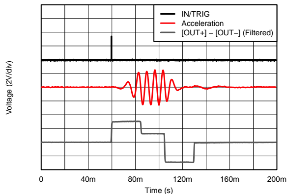
V_{DD} = 3.6\text{ V} ERM open loop Strong click - 60% External edge trigger
