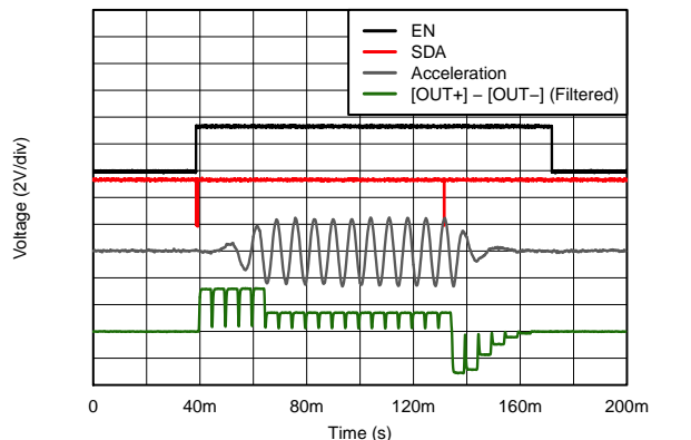
V_{DD} = 3.6\text{ V} ERM closed loop RTP Mode
