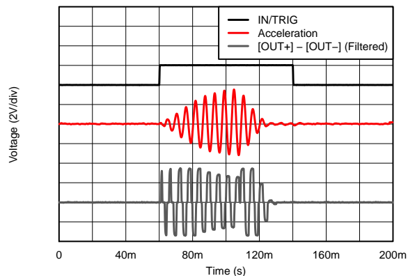
V_{DD} = 3.6\text{ V} LRA closed loop Strong click - 100% External level trigger
