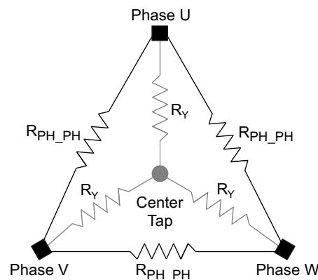
图 14. Delta-Connected Motor and the Equivalent Wye Connections
