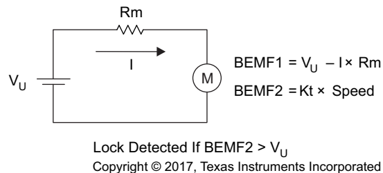
图 35. Lock Detection 1
