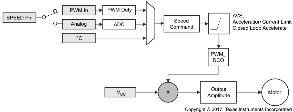
图 8-3. Multiplexing the Speed Command to the Output Amplitude Applied to the Motor
