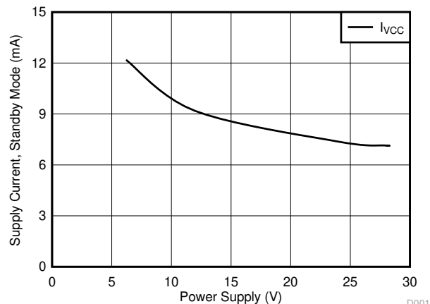
图 7-5. Supply Current vs Power Supply Voltage
