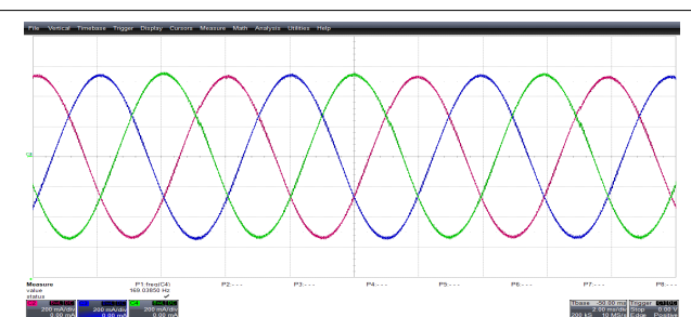
图 9-3. DRV10982-Q1 Operation Current Waveform
