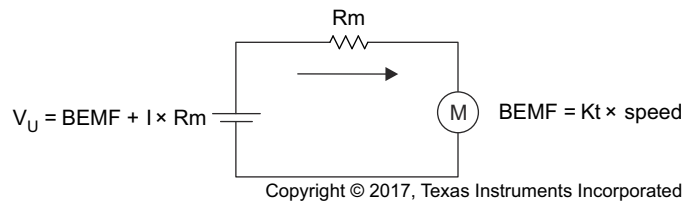
图 8-19. Motor Start-Up Current
