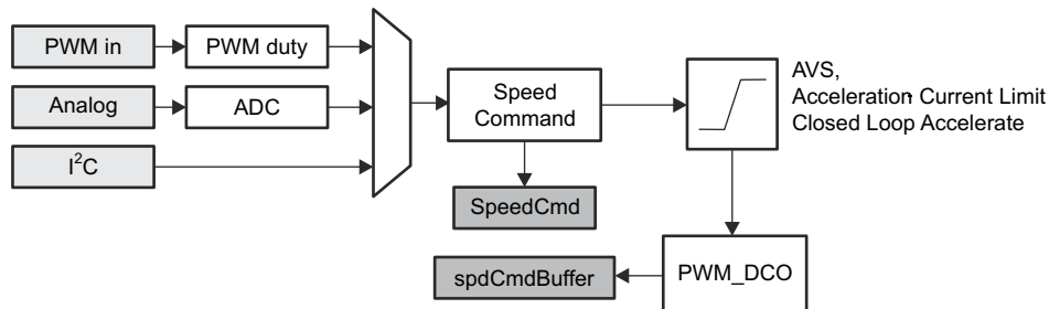
图 8-38. SpeedCmd and spdCmdBuffer Registers
