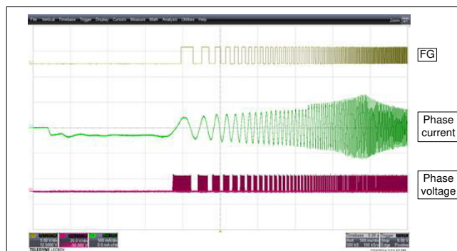
图 9-2. DRV10982-Q1 Start-Up Waveform
