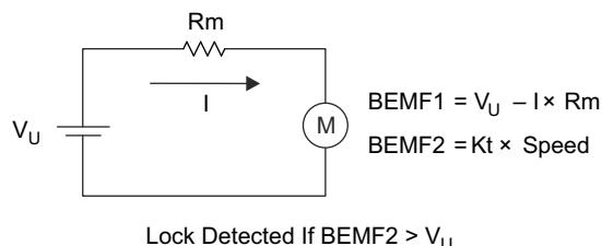
图 8-29. Lock Detection 1
