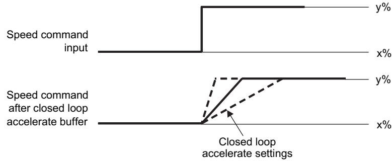
图 25. Closed-Loop Accelerate
