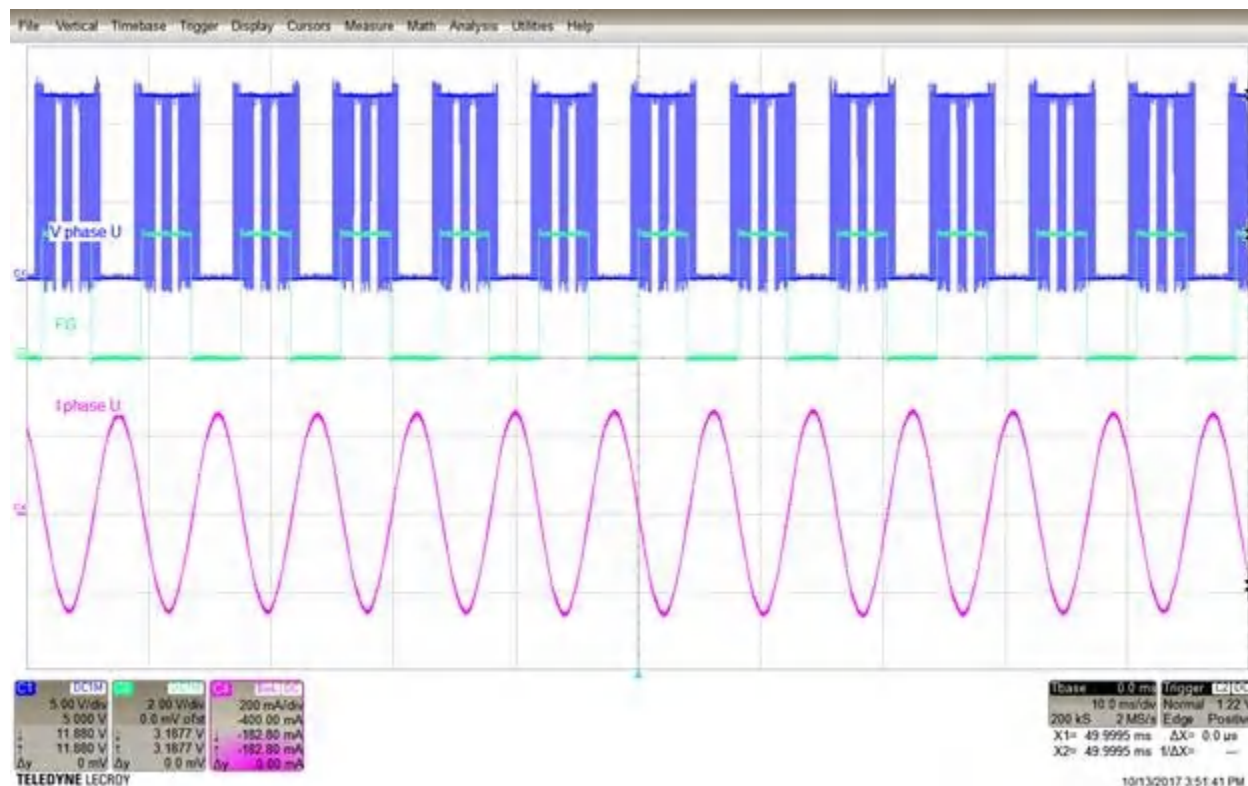
图 7-1. 180° Sensorless-Control Scheme
