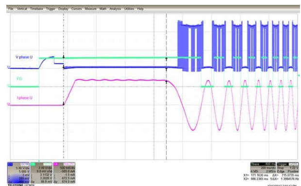
图 8-3. DRV10974 Start-Up Waveform
