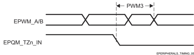
图 6-60. EPWM_A/B and ePWM_TZn_IN Forced High/Low Input Timings
