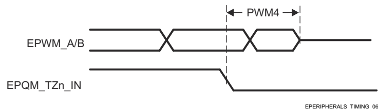
图 6-61. EPWM_A/B and ePWM_TZn_IN Hi - Z Input Timings
