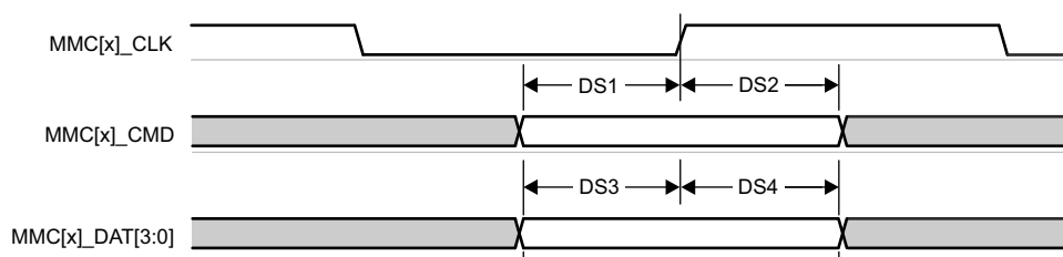
图 6-97. MMC1/2 – Default Speed – Receive Mode
