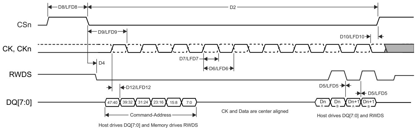
图 6-79. HyperBus Timing Diagrams - Receiver Mode
