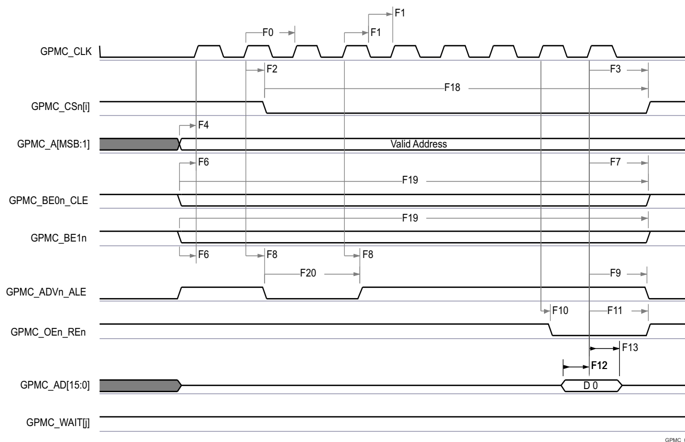
图 6-63. GPMC and NOR Flash — Synchronous Single Read (GPMCFCLKDIVIDER = 0)
