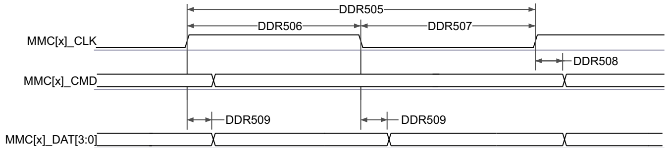
图 6-106. MMC1/2 - UHS-I DDR50 - Transmit Mode
