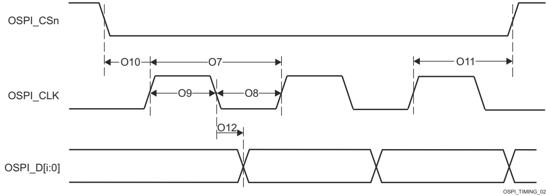
图 6-112. OSPI Switching Characteristics - SDR
