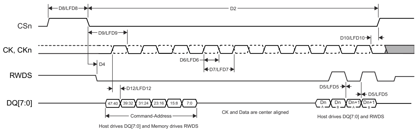
图 7-72. HyperBus Timing Diagrams - Transmitter Mode
