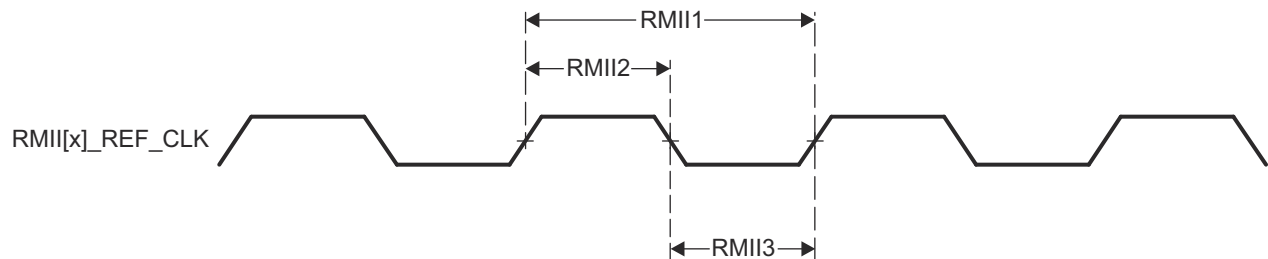
图 7-45. RMII[x]_REFCLK Timing - RMII Mode
