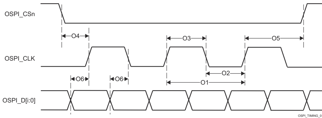
图 7-104. OSPI Switching Characteristics - DDR
