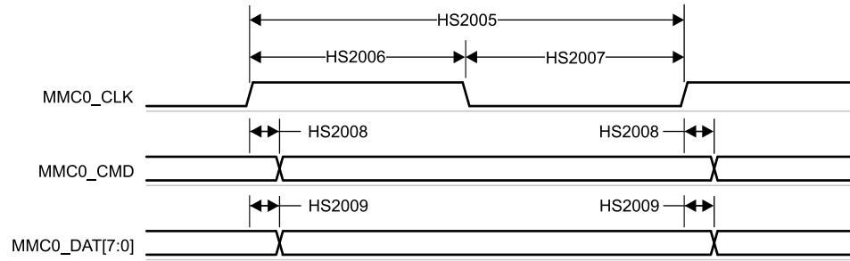
图 7-89. MMCSD0 - HS200 Mode - Transmit Mode
