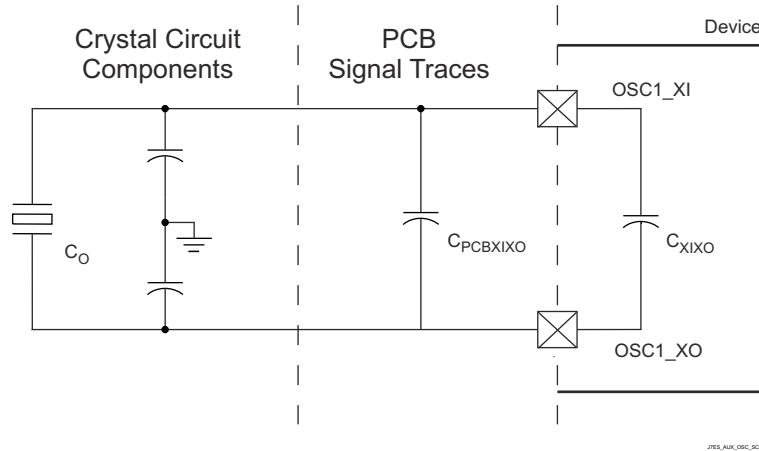
图 7-32. Shunt Capacitance
