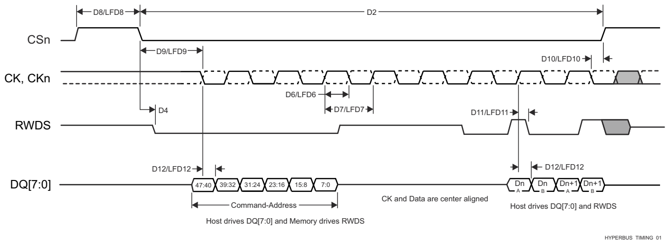
图 7-72. HyperBus Timing Diagrams - Transmitter Mode
