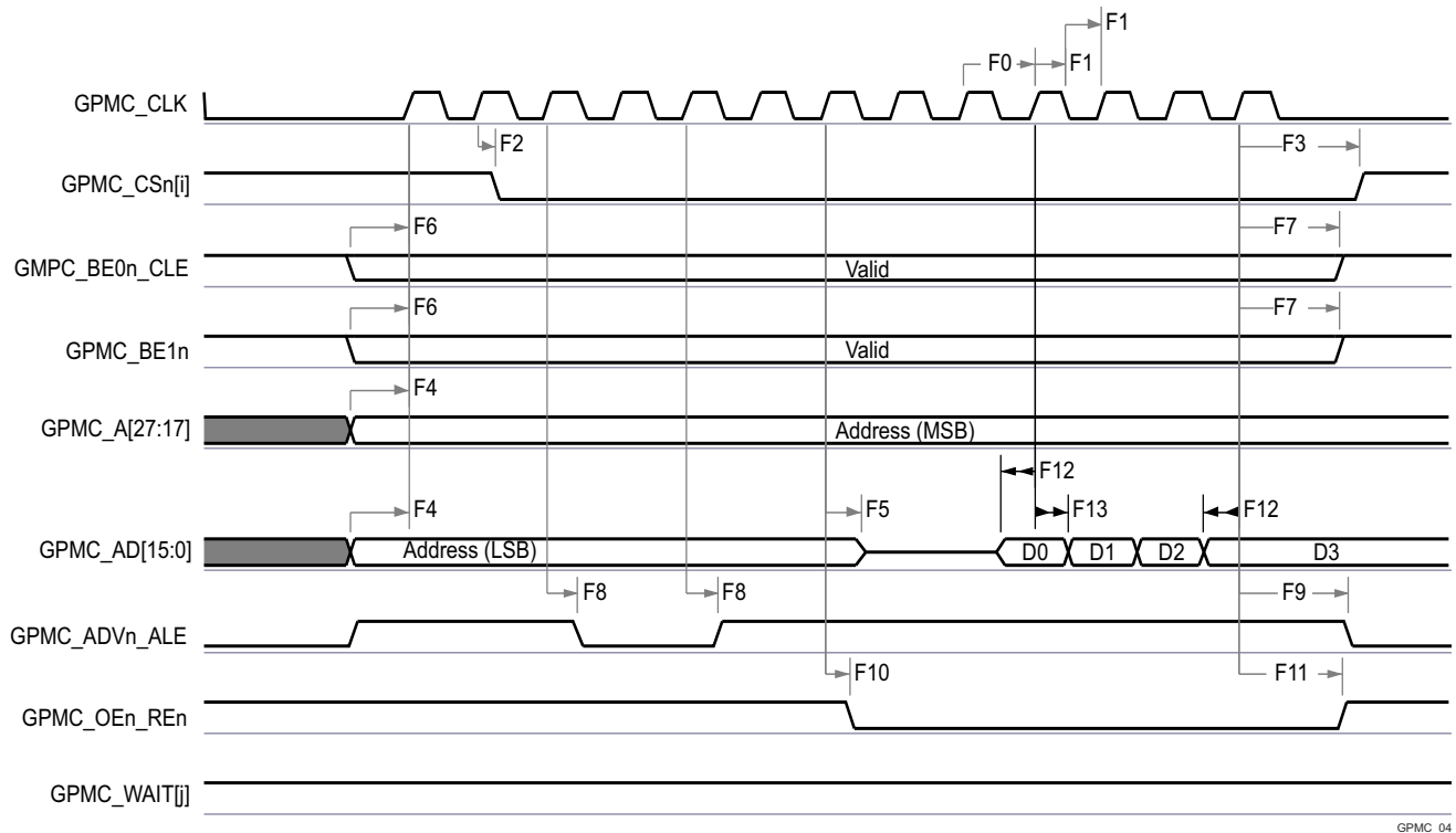
图 7-59. GPMC and NOR Flash—Synchronous Burst Write (GPMCFCLKDIVIDER = 0)
