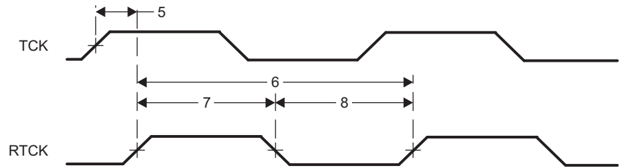
图 5-131. JTAG With RTCK Timing
