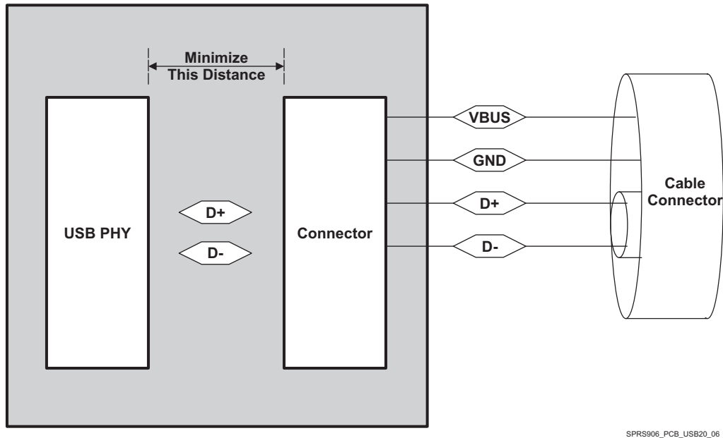
图 7-26. USB PHY Connector and Cable Connector
