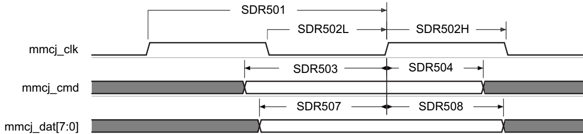
图 5-107. MMC/SD/SDIOj in - High Speed SDR50 - Receiver Mode
