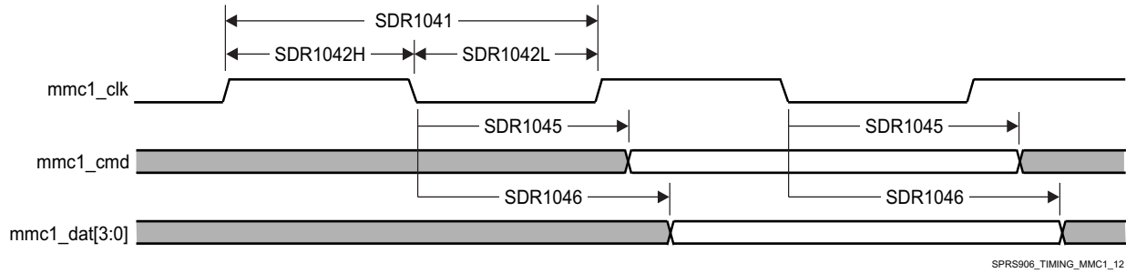
图 5-89. MMC/SD/SDIO in - High Speed SDR104 - Transmitter Mode
