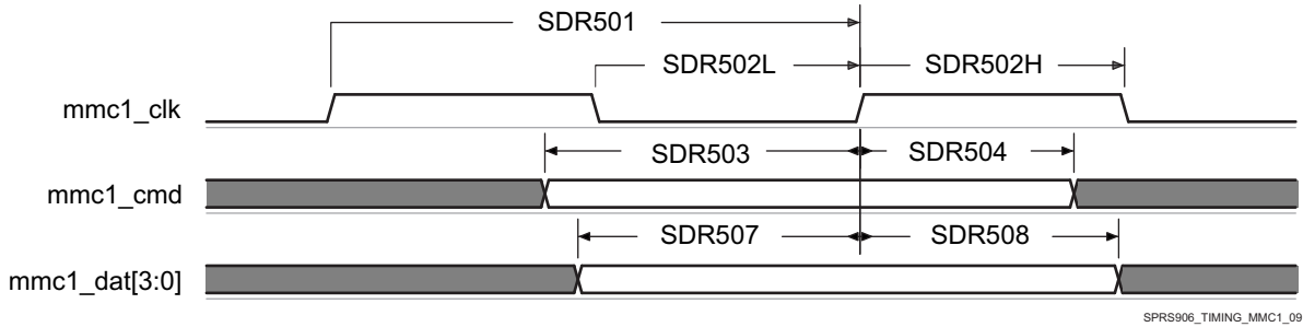
图 5-86. MMC/SD/SDIO in - High Speed SDR50 - Receiver Mode
