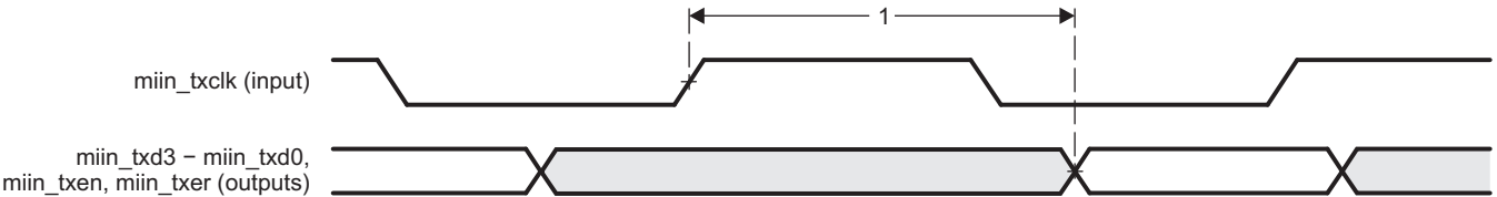
图 5-71. GMAC Transmit Interface Timing MIIn operation
