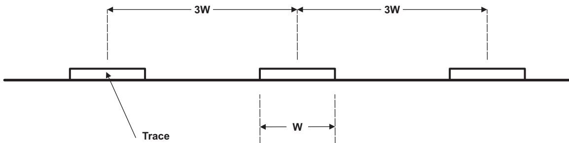
图 7-24. 3W Spacing Rule
