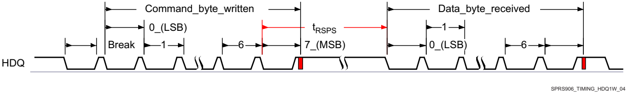
图 5-44. HDQ Communication Timing
