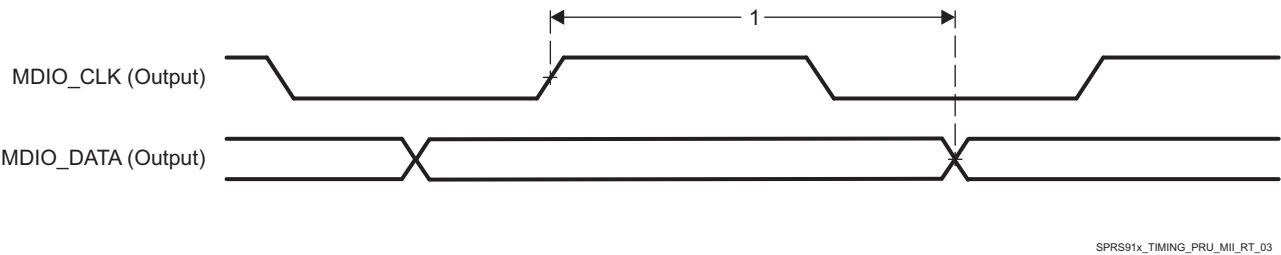
图 5-124. PRU-ICSS MDIO_DATA Timing – Output Mode
