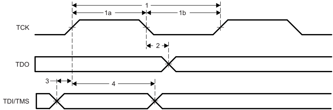
图 5-130. JTAG Timing
