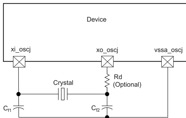
图 7-22. Grounding Scheme for High-Frequency Clock
