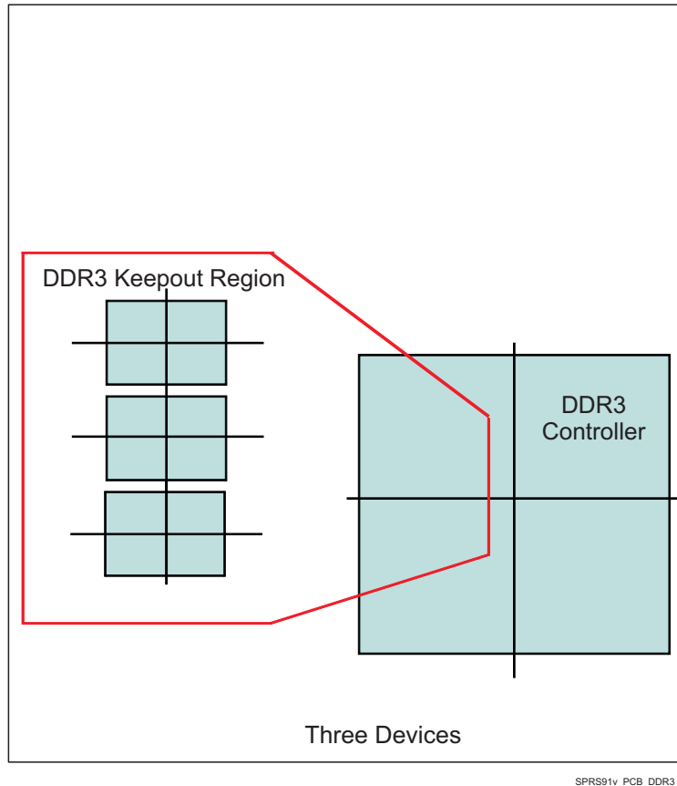
图 7-34. DDR3 Keepout Region
