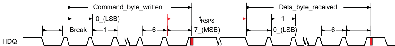
Figure 5-44. HDQ Communication Timing
