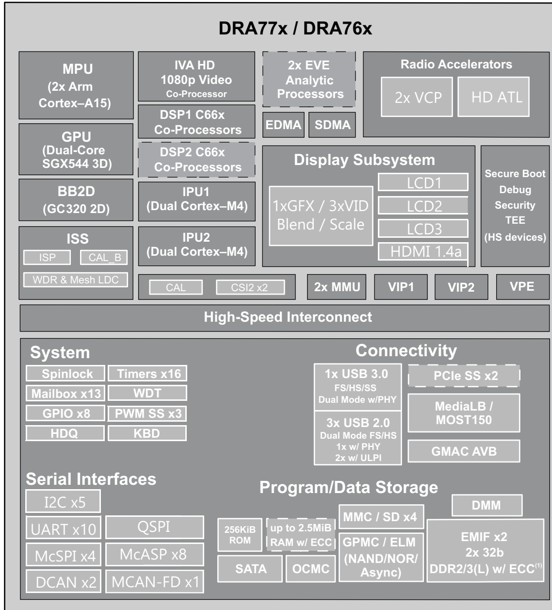
图 6-1. DRA77x, DRA76x Block Diagram
