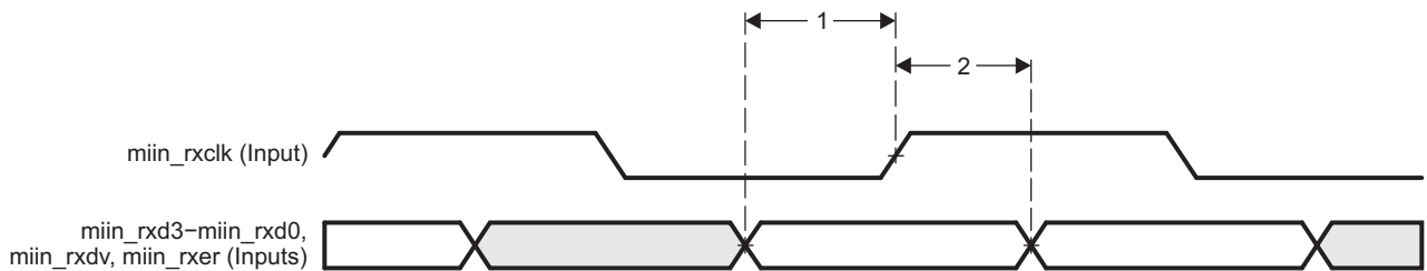
Figure 5-70. GMAC Receive Interface Timing MIIn Operation
