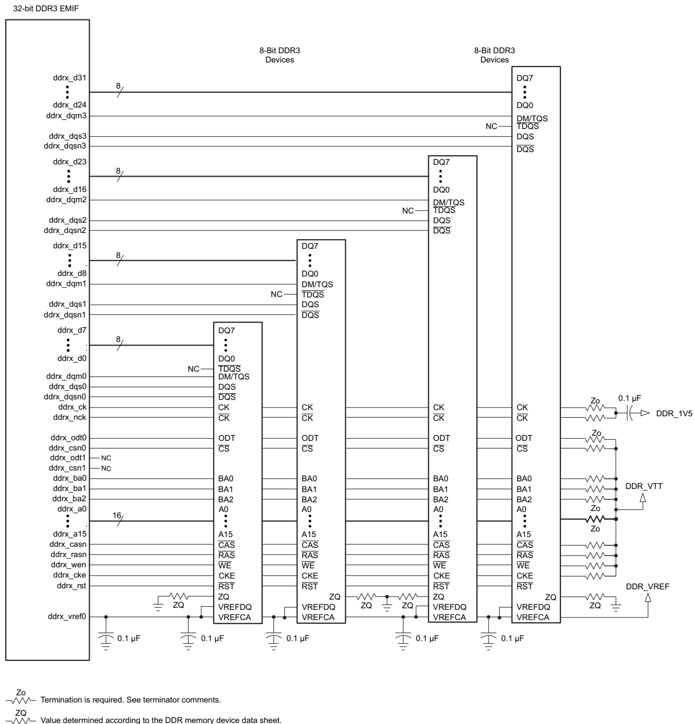
图 7-56. 32-Bit, One-Bank DDR3 Interface Schematic Using Four 8-Bit DDR3 Devices
