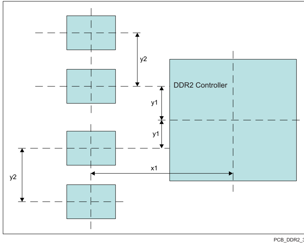
图 7-49. Device and DDR2 Device Placement
