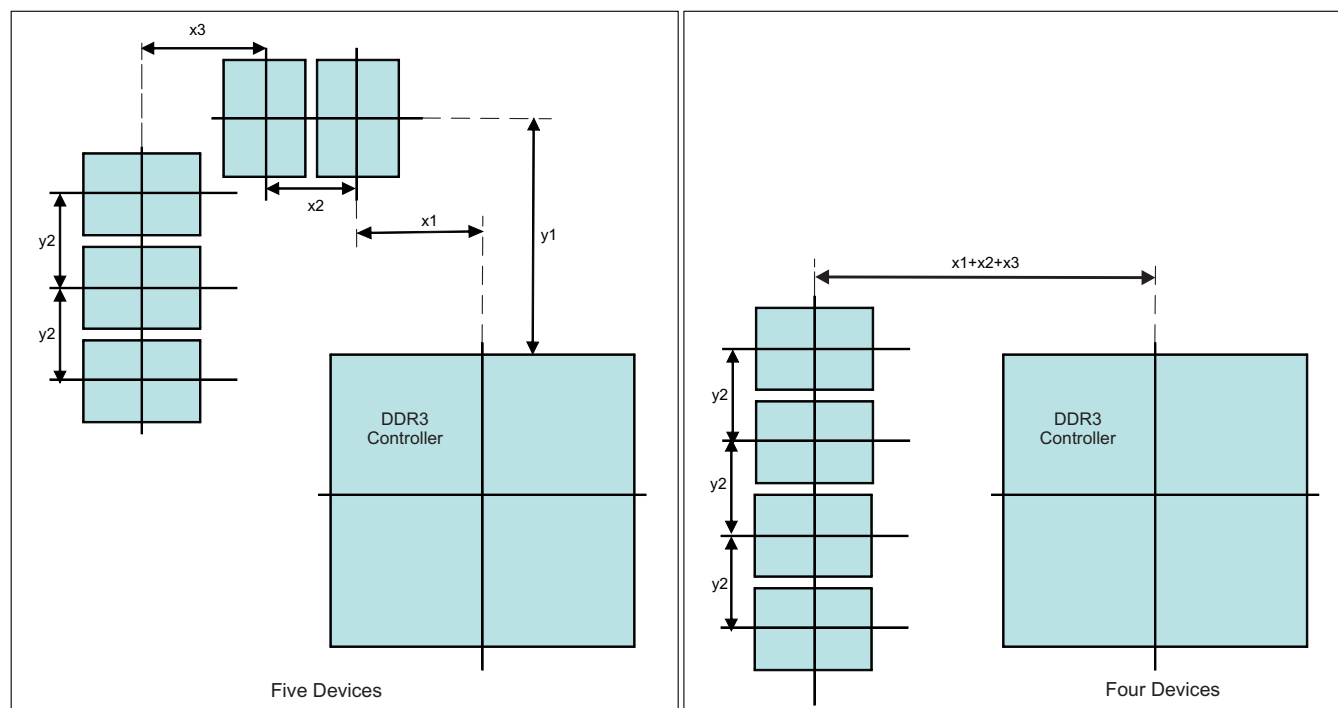
图 7-57. Placement Specifications
