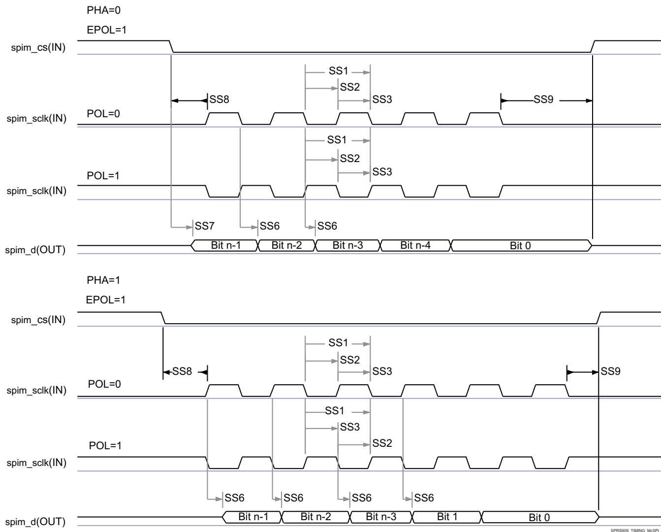
Figure 5-51. McSPI - Slave Mode Transmit
