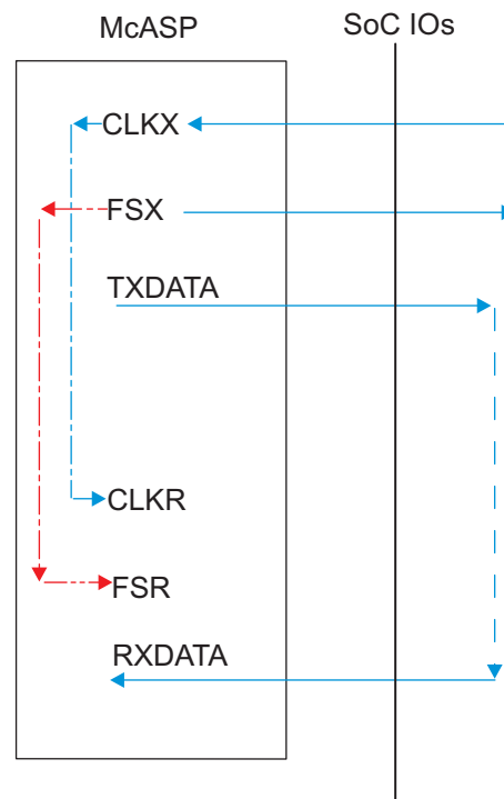
Figure 5-64. McASP1-8 CI-FO- – SYNC Mode
