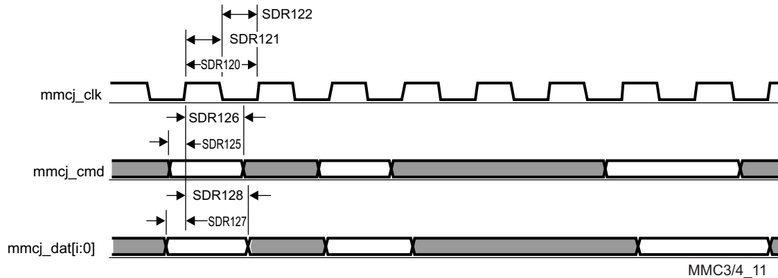
Figure 5-103. MMC/SD/SDIOj in - SDR12 - Receiver Mode
