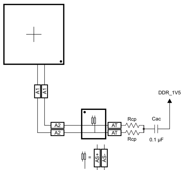
图 7-73. CK Routing for One DDR3 Device
