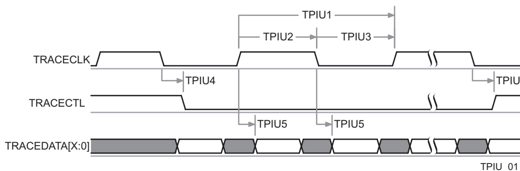
图 5-112. TPIU—PLL DDR Transmit Mode (1)
