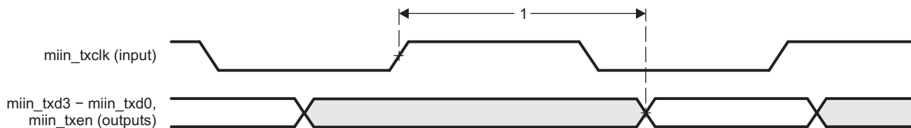
Figure 5-71. GMAC Transmit Interface Timing MIIn Operation
