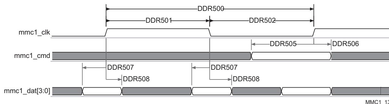
Figure 5-90. SDMMC - High-Speed SD - DDR - Data/Command Receive
