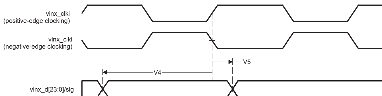
Figure 5-21. Video Input Ports timings
