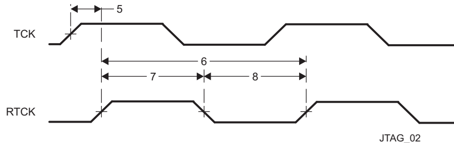
图 5-116. JTAG With RTCK Timing
