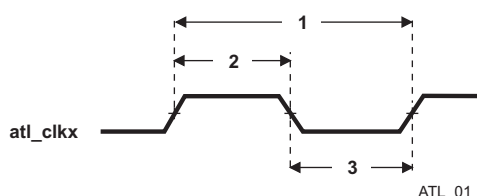
Figure 5-114. ATL_CLKOUTx Timing
