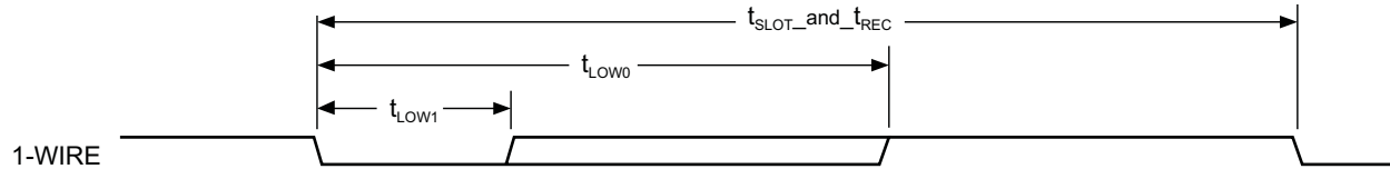
图 7-31. 1-Wire—Write Bit-One Timing (Command / Address or Data)
