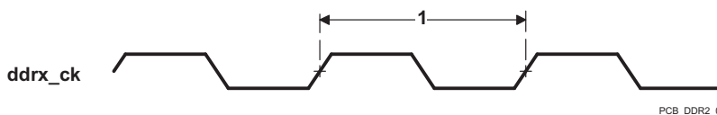
图 8-49. DDR2 Memory Controller Clock Timing
