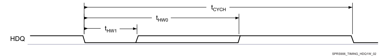
图 7-26. Device HDQ Interface Bit Read Timing (Data)
