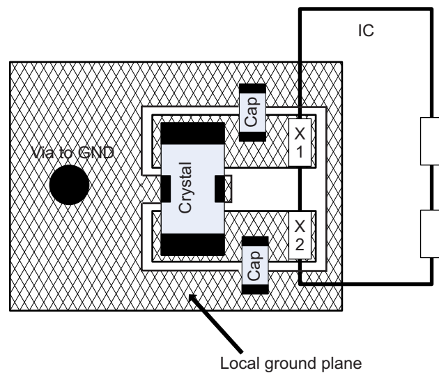
图 8-37. Slow Clock PCB Requirements
