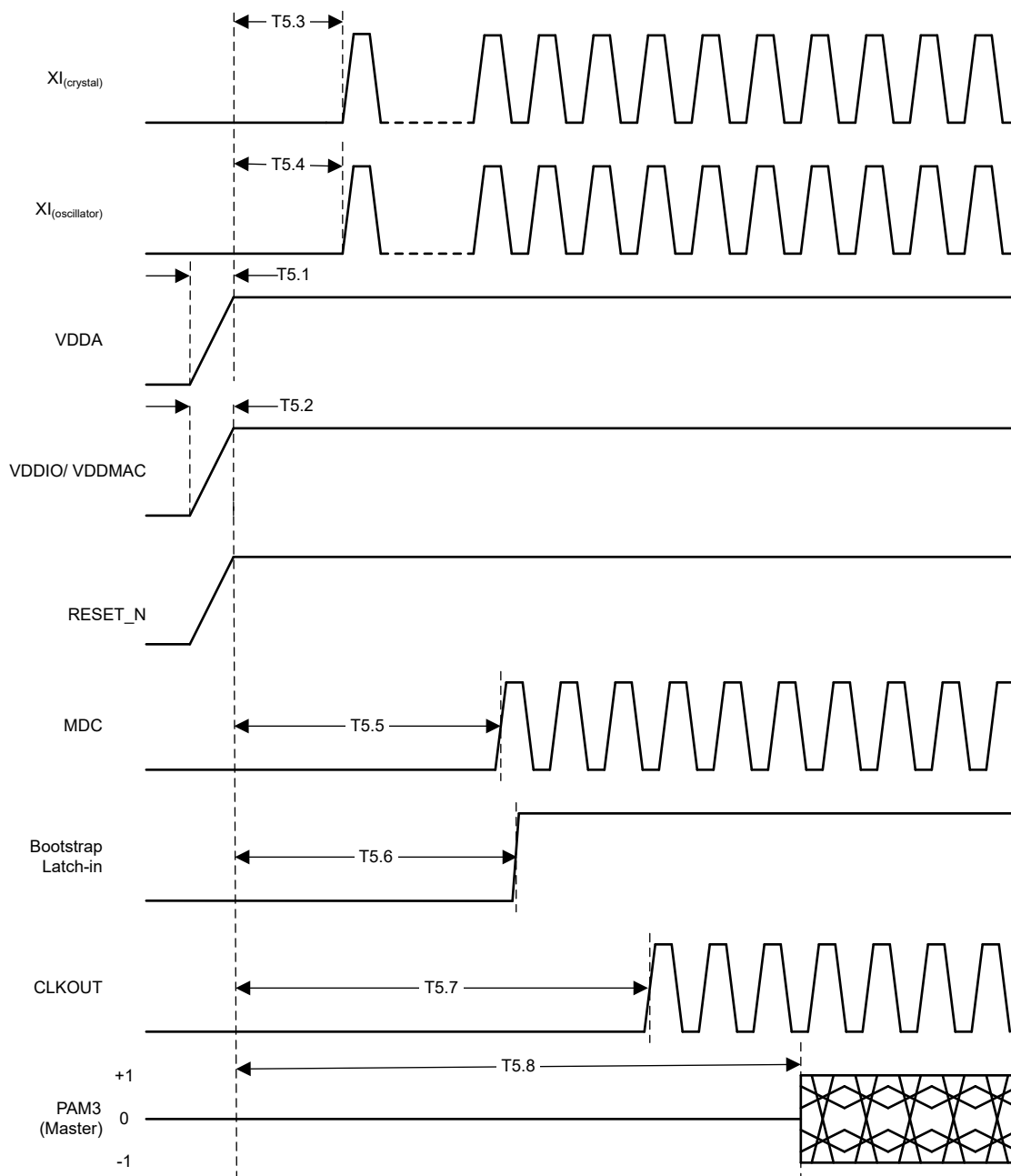
图 7-8. Power-Up Timing
