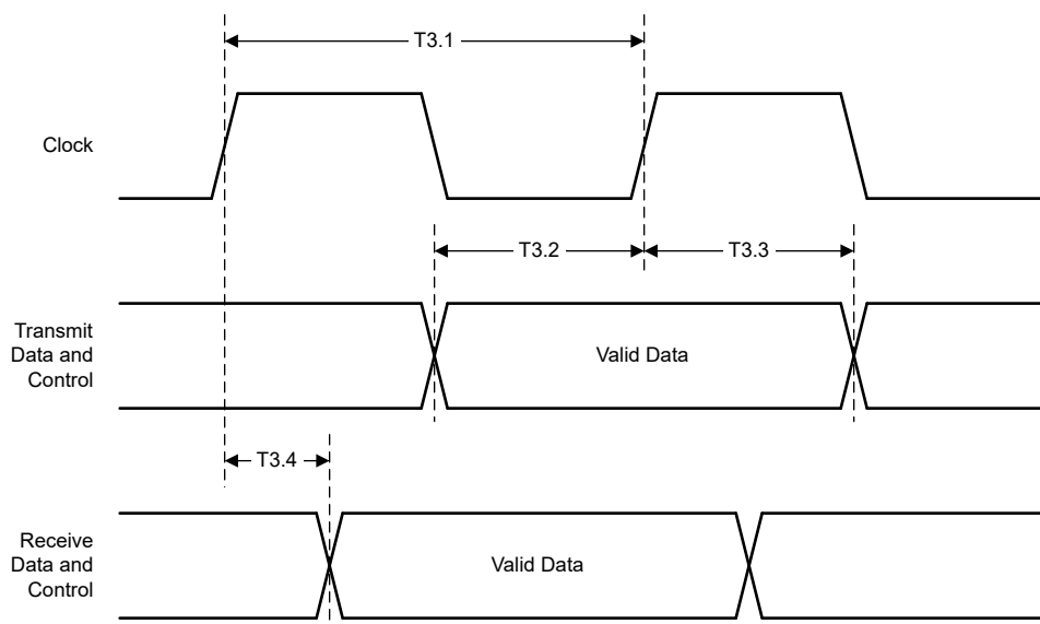
图 6-2. RMI Transmit and Receive Timing
