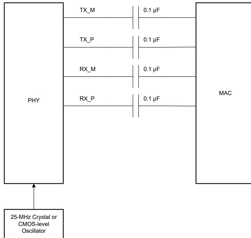
图 7-17. SGMII Connections
