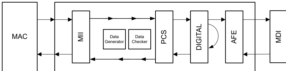
图 7-6. Digital loopback without data generator
