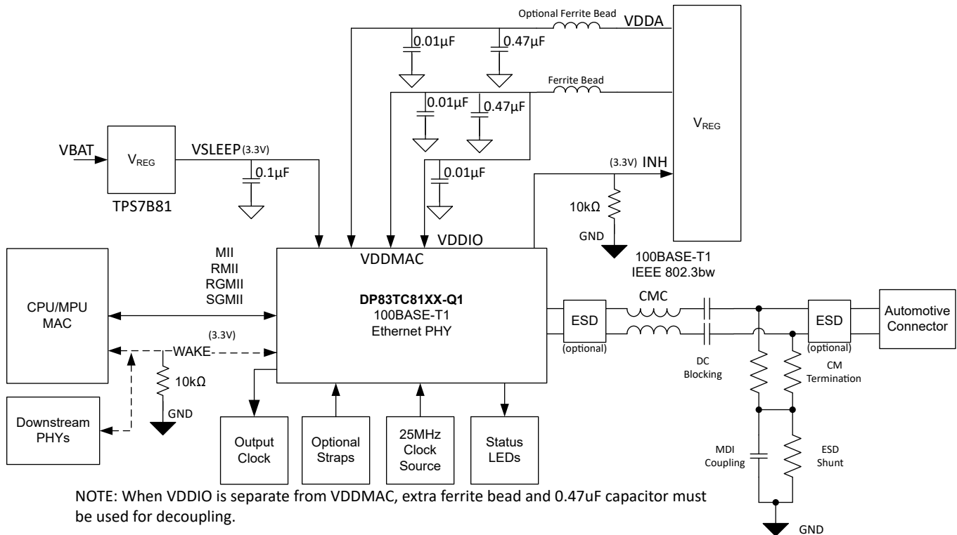
图 8-9. Typical TC-10 Application With Peripherals
