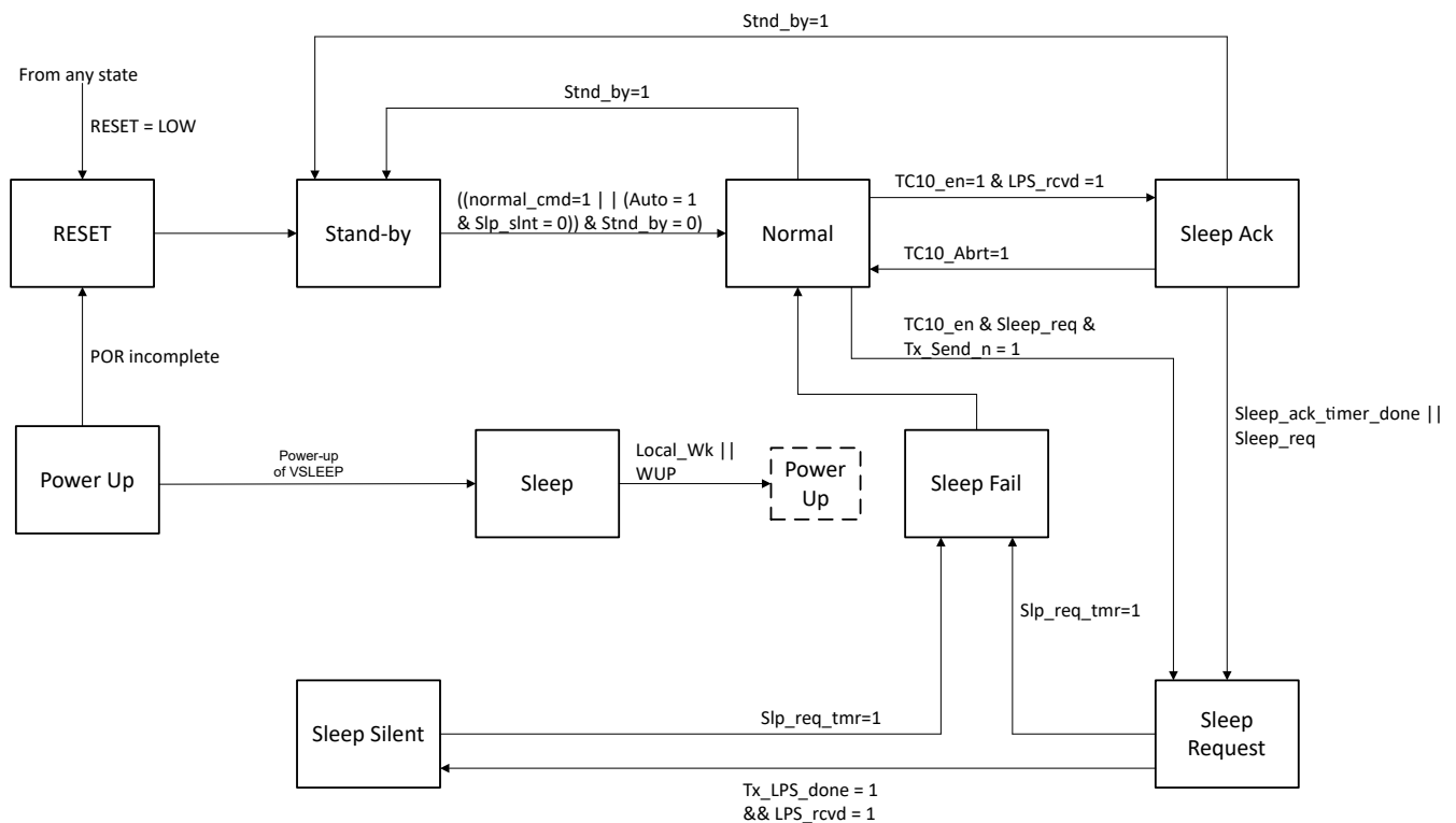
图 7-11. PHY Operation State Diagram
