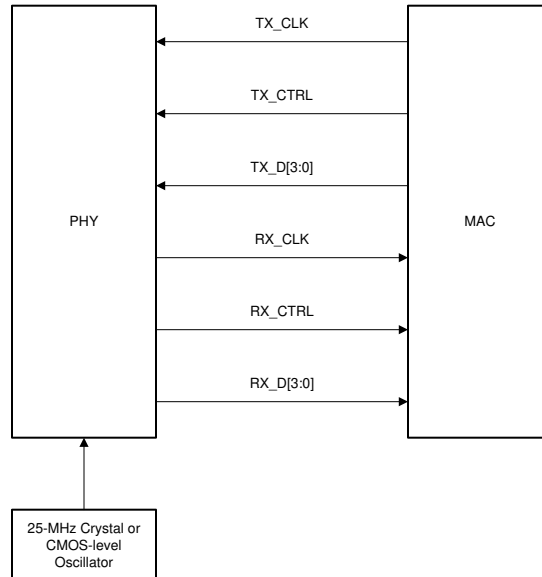
图 7-16. RGMII Connections
