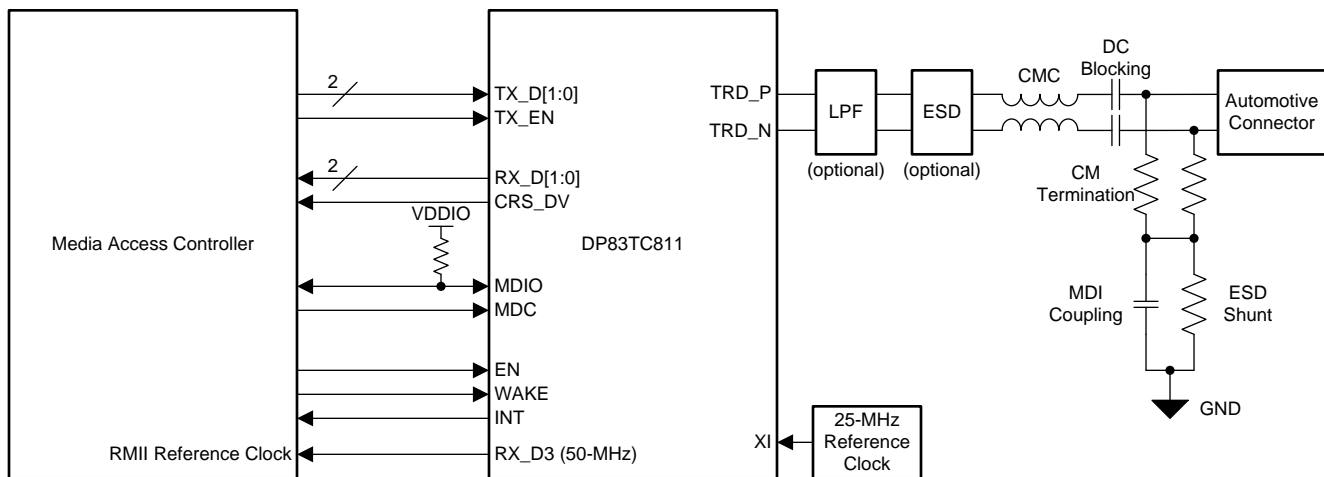
图 134. Typical Application (RMII Master)
