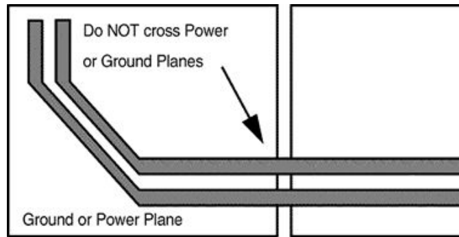
图 8-13. Differential Signal Pair-Plane Crossing
