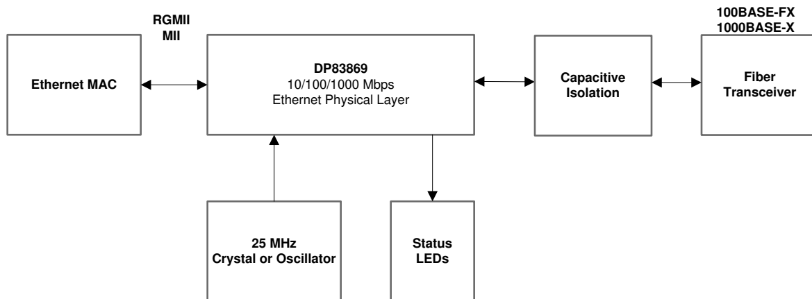
图 8-6. Typical Fiber Ethernet Application
