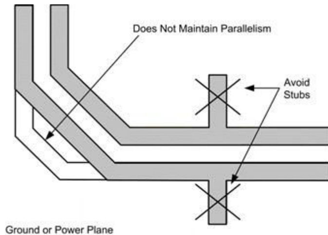
图 8-12. Avoiding Stubs in a Differential Signal Pair
