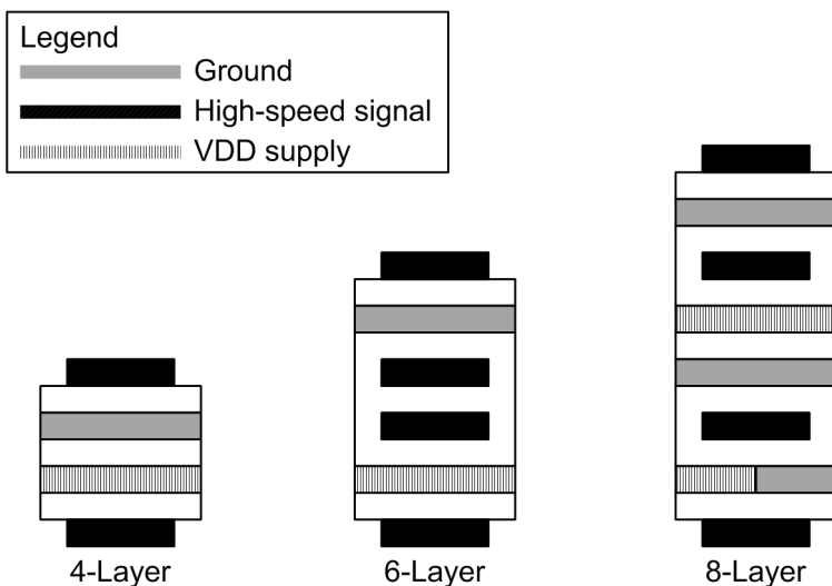
图 8-14. Recommended Layer Stack-Up
