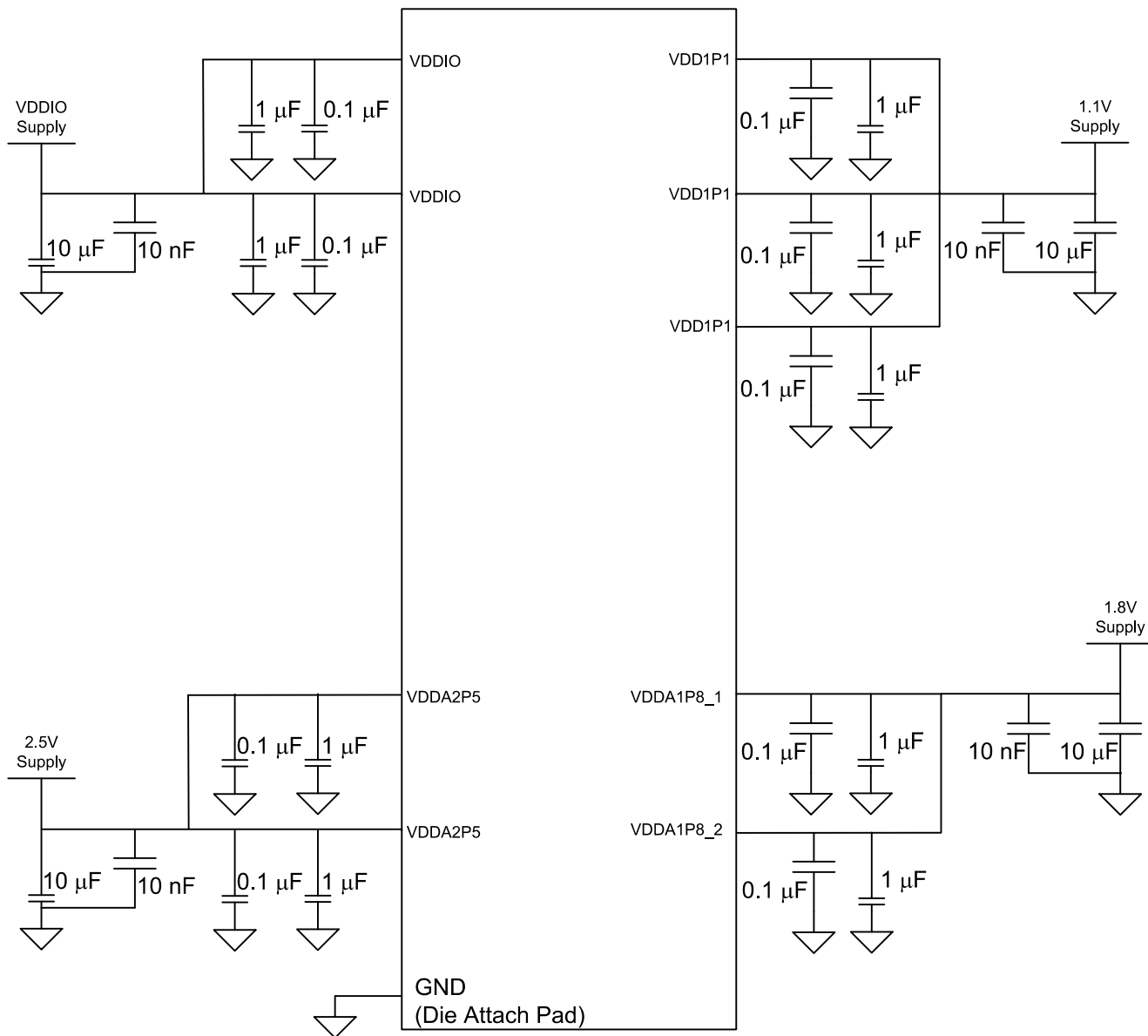
图 8-10. Three-Supply Configuration
