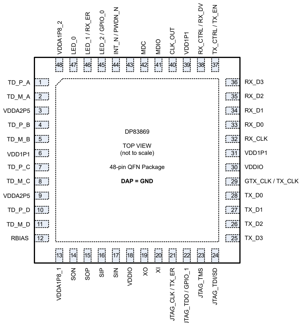
图 5-1. RGZ Package (48-Pin VQFN) Top View
