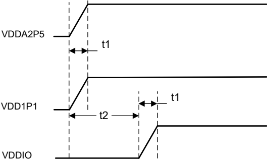
图 8-9. Two-Supply Sequence Diagram
