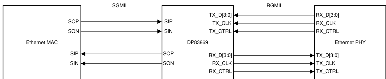
图 7-10. DP83869HM SGMII-to-RGMII Bridge
