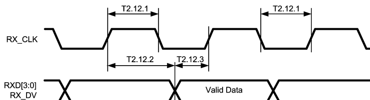
Figure 5-12. 10 Mb/s MII Receive Timing
