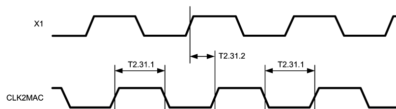
Figure 5-29. 25 MHz_OUT Timing
