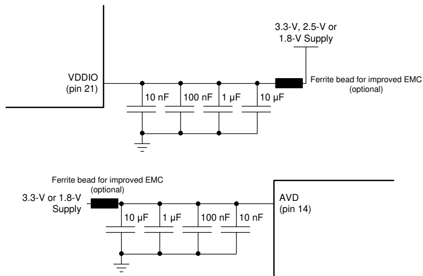
图 10-1. Power Connections
