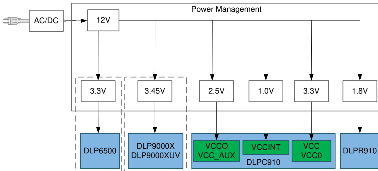
图 9-1. Power Distribution
