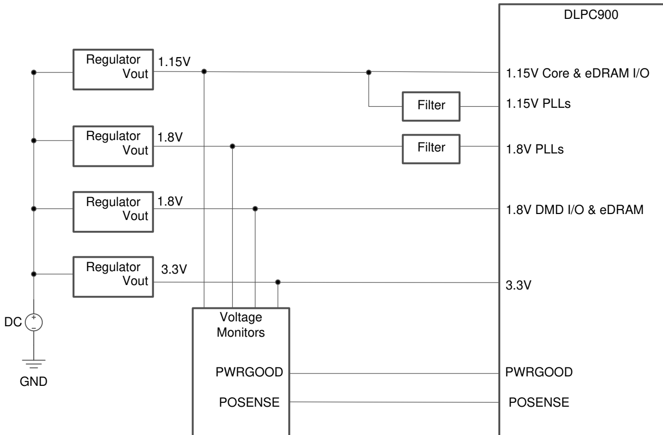
图 8-1. Power Regulation
