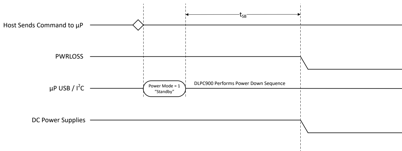
图 5-4. Anticipated Power Down Timing Diagram
