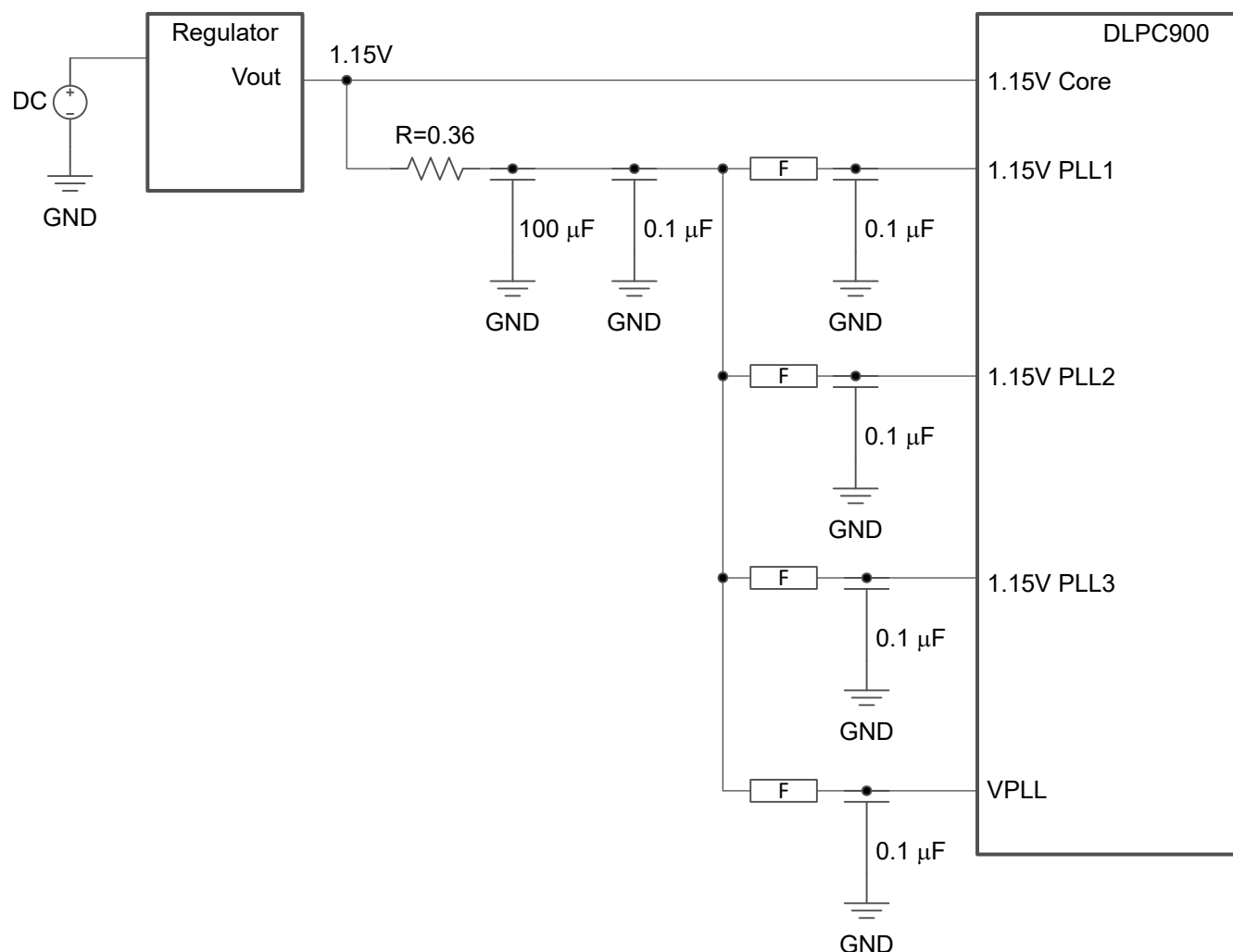
图 9-1. Recommended Filter Topology for PLL 1.15V Supplies
