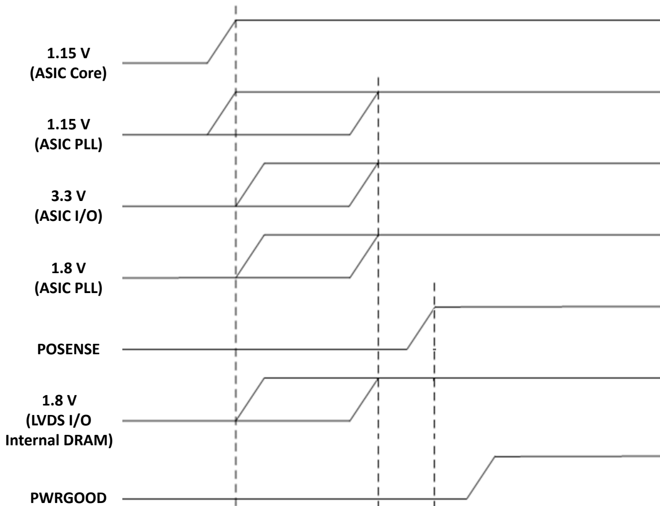
图 8-2. Power Sequencing
