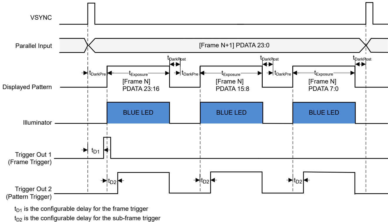
图 7-8. 3 \times 8 -bit (Blue) Pattern Configurations
