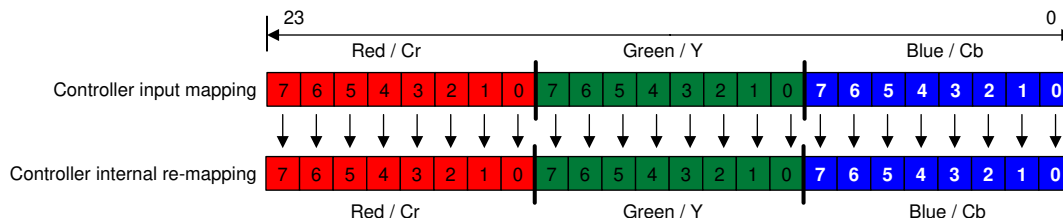
图 7-2. RGB-888 and YCbCr-888 I/O Mapping
