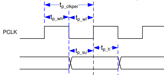
图 5-8. Parallel Interface Pixel Timing
