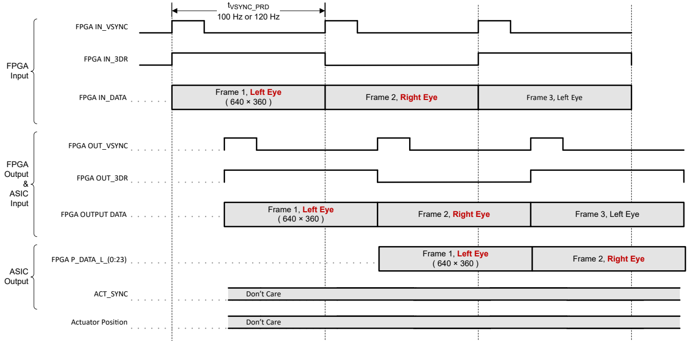
图 6-2. 3D Frame and Signal Timing
