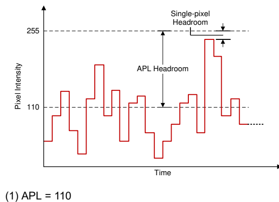
图 6-8. Source Pixels for a Color Channel
