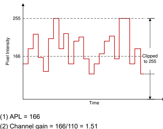
图 6-9. Pixels for a Color Channel After CAIC Processing
