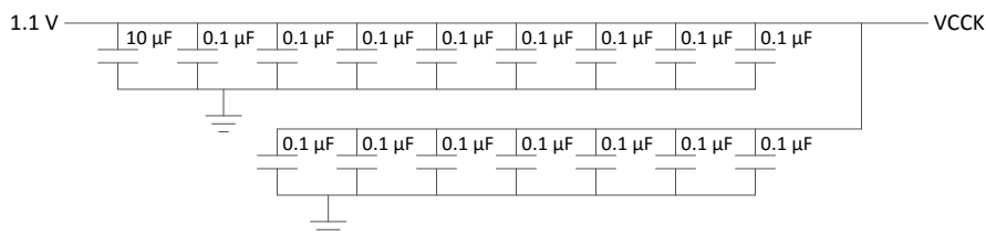
图 8-3. VCCCK Recommended Filter
