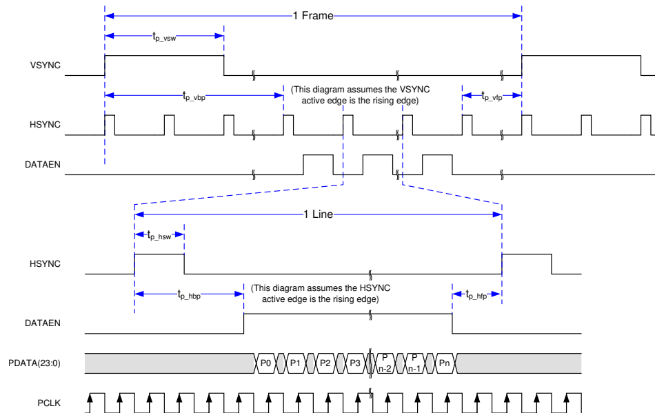
图 5-5. Source Frame Timing
