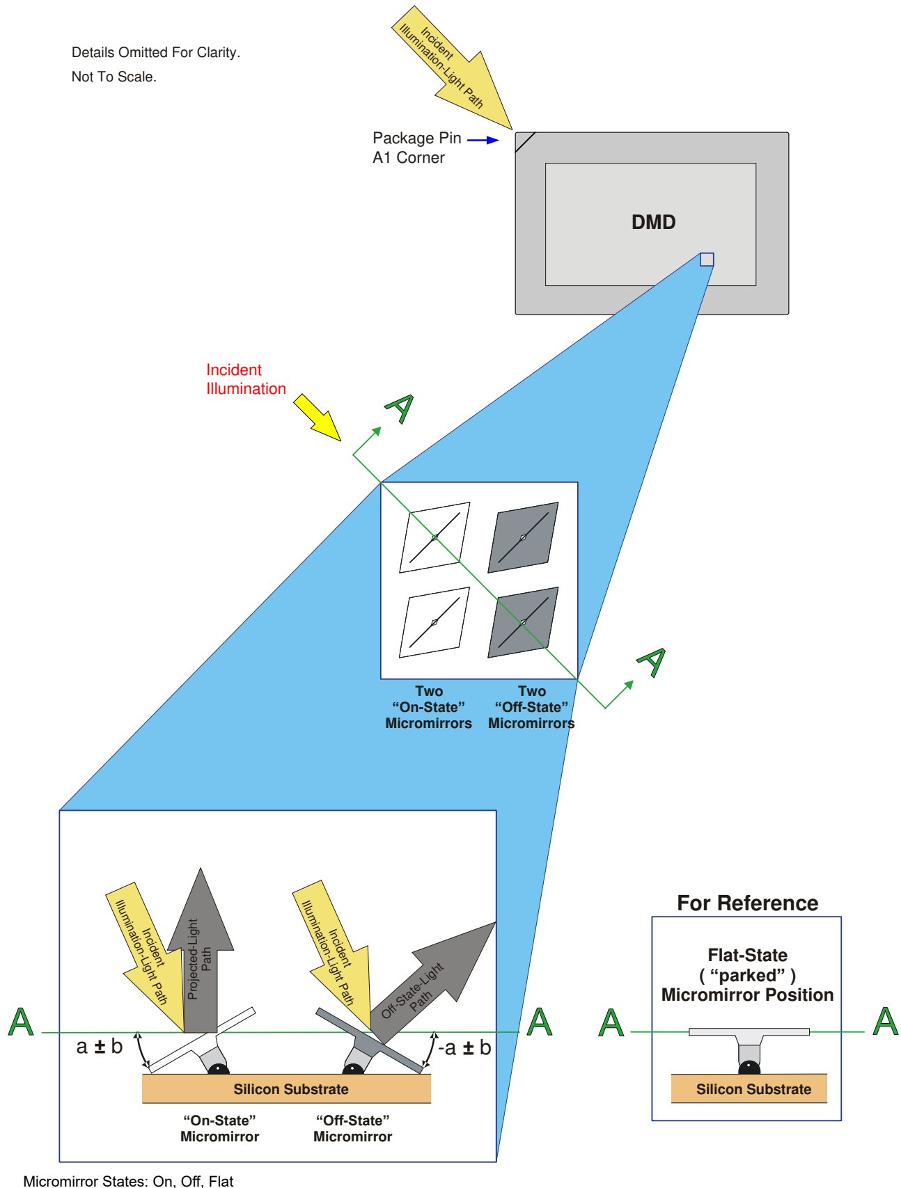
图 7-3. Micromirror States: On, Off, Flat
