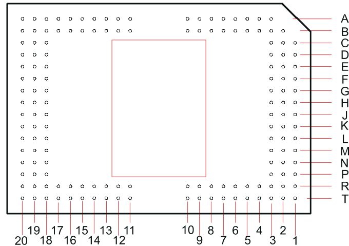
图 5-1. FYA Package 149-Pin CPGA Series 450 Bottom View
