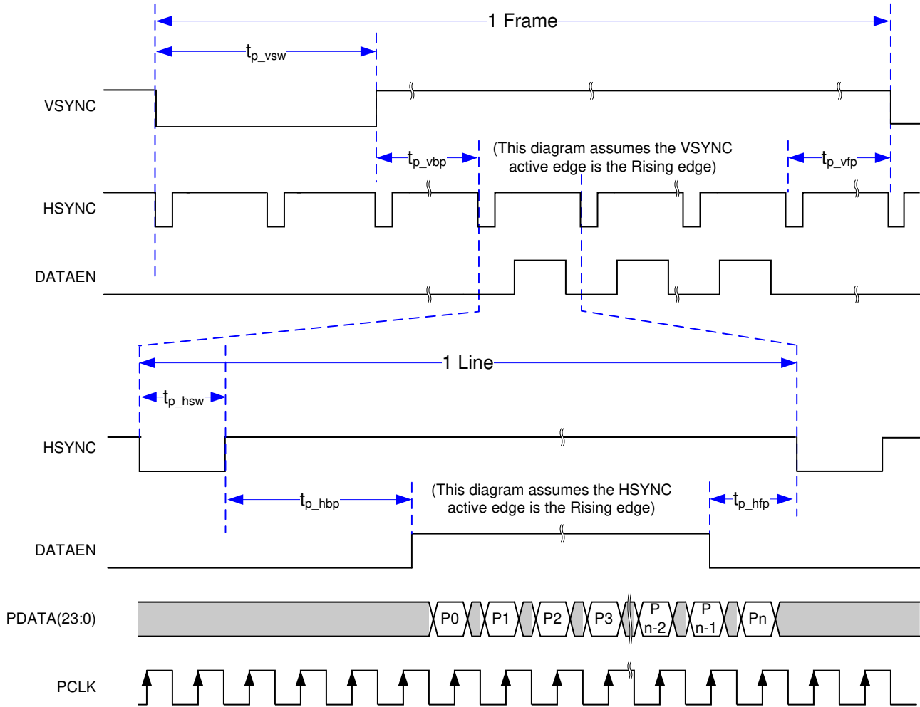
图 6-4. Parallel Interface Frame Timing
