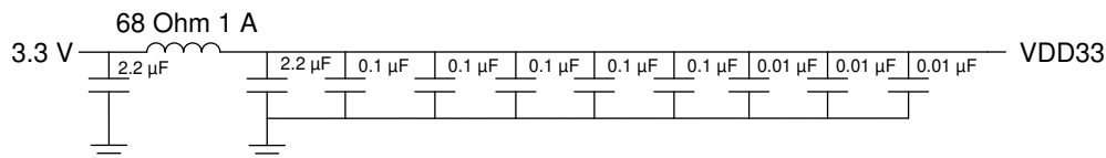
图 10-4. VDD33 Recommended Filter
