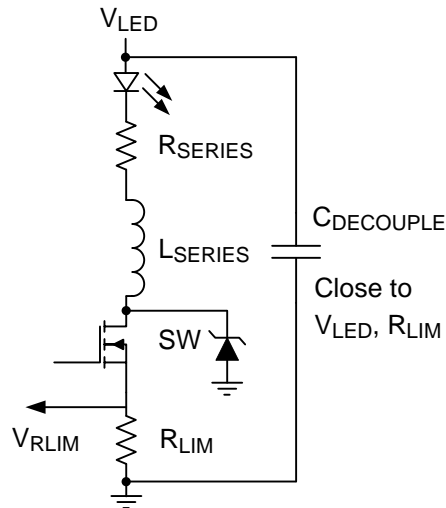
图 32. Parasitic Inductance ( L_{\text{Series}} ) and Resistance ( R_{\text{series}} ) in Series with LED
