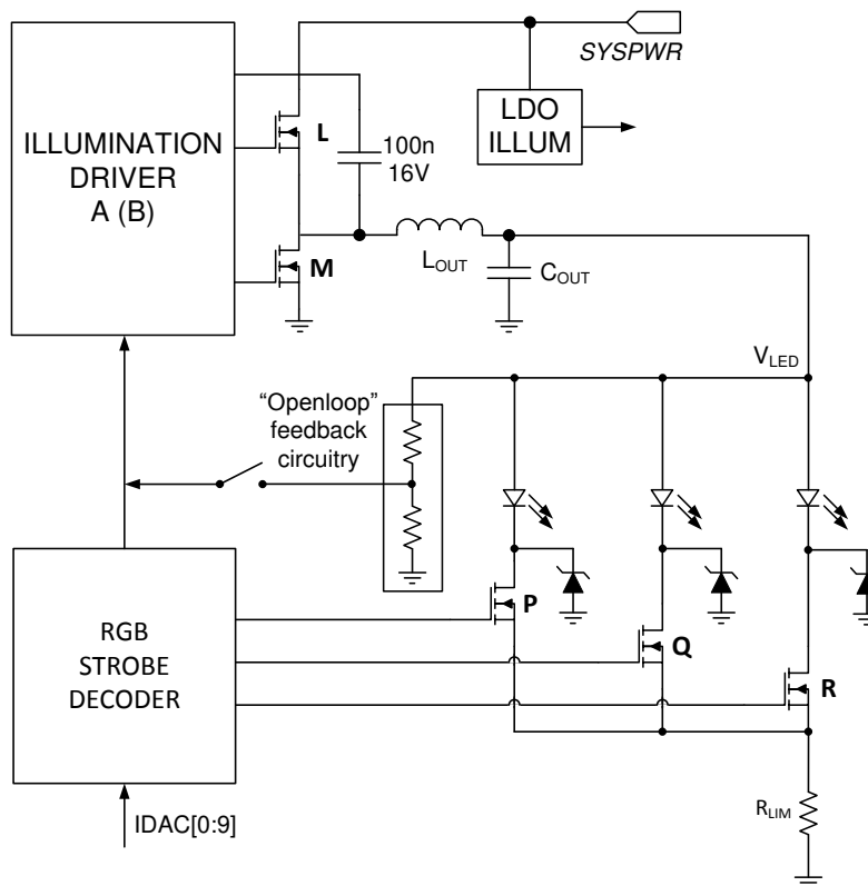
图 8-4. Illumination Control Loop
