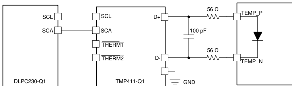
图 7-1. Temperature Sense Diode Typical Circuit Configuration
