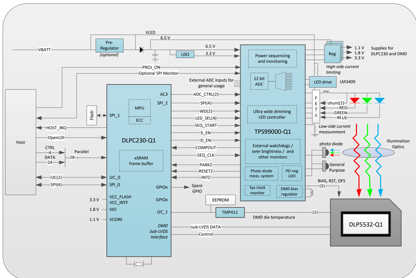
图 8-1. Window Display System Block Diagram
