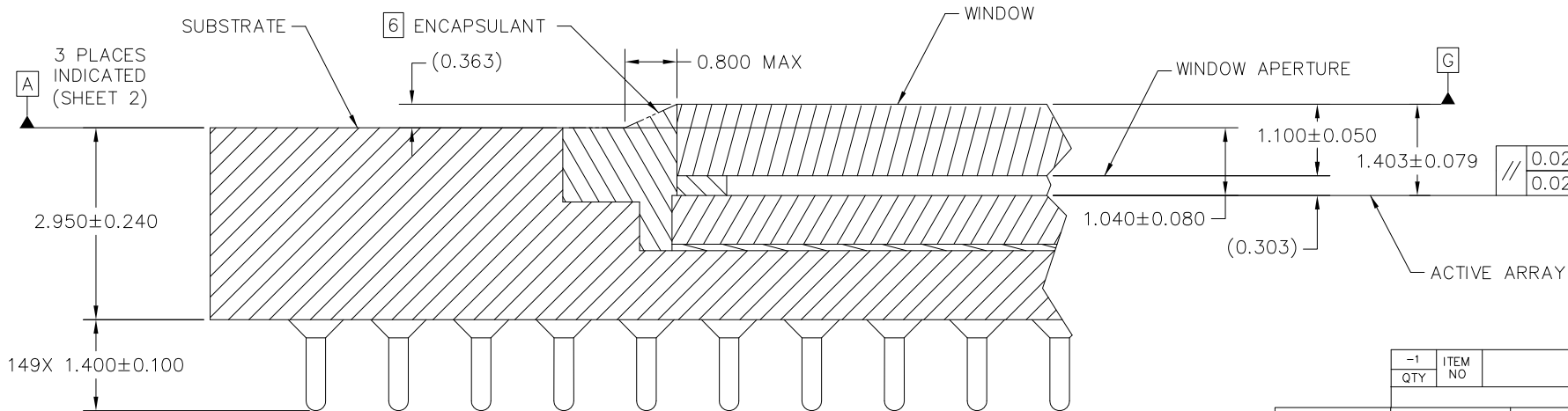
SECTION A-A SCALE 20/1
