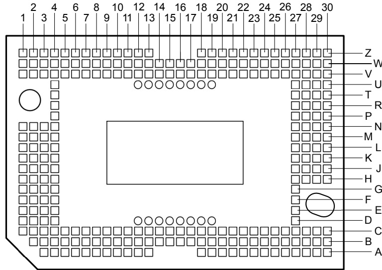
图 4-1. Series 410 257-pin FXH Bottom View
