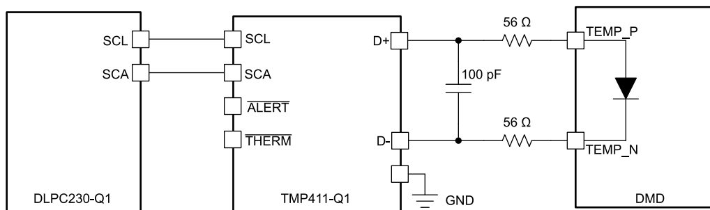
图 6-1. Temperature Sense Diode Typical Circuit Configuration
