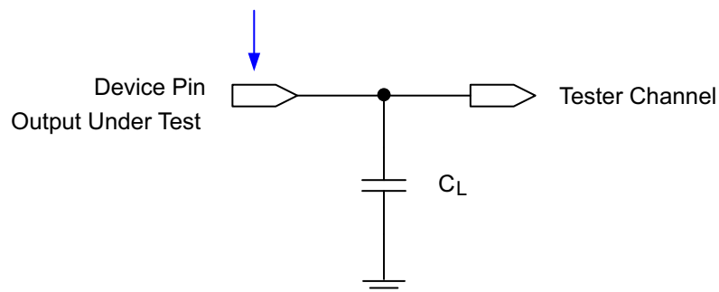
图 6-13. Test Load Circuit for Output Propagation Measurement
