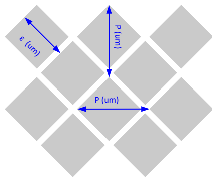
图 6-8. Mirror (Pixel) Pitch
