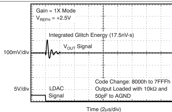
Figure 63. Major Carry Glitch
