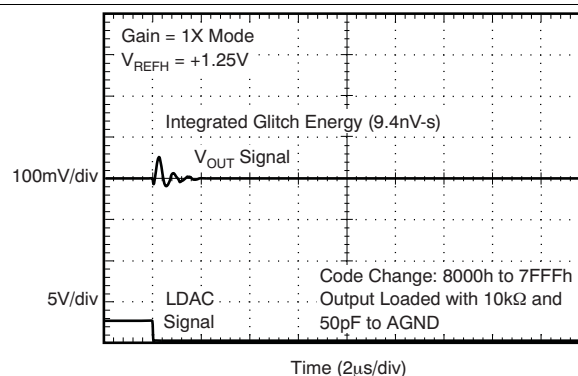
Figure 65. Major Carry Glitch
