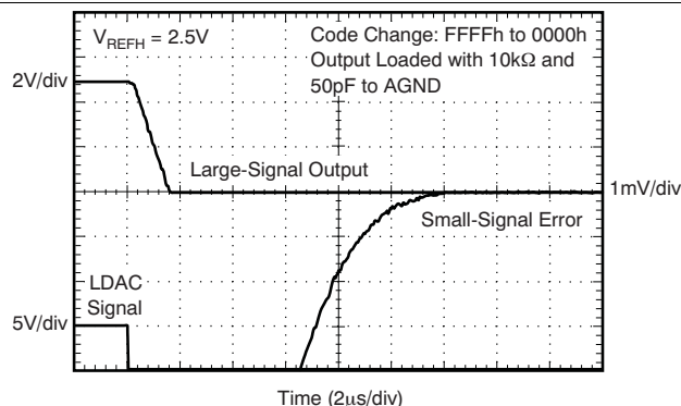
Figure 35. Large Signal Settling Time (Gain = 2X MI)
