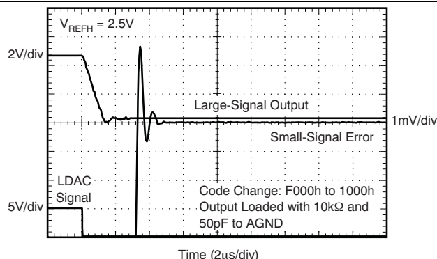
Figure 37. Large Signal Settling Time (Gain = 2X Mode)
