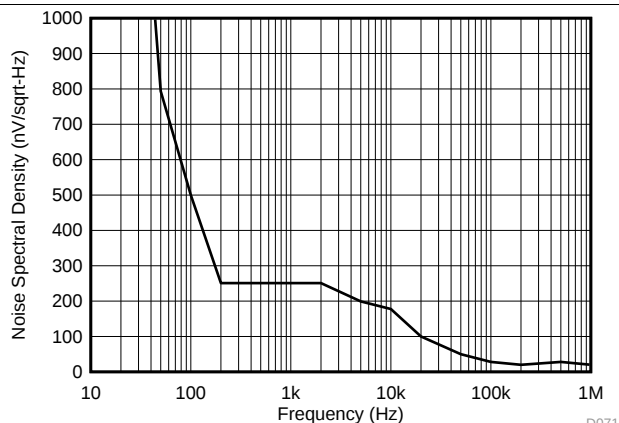
图 75. Internal Reference Voltage Noise Spectral Density (DC/DC Enabled)
