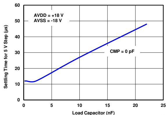
图 7-36. VOUT Settling Time vs Load (No Compensation Capacitor)
