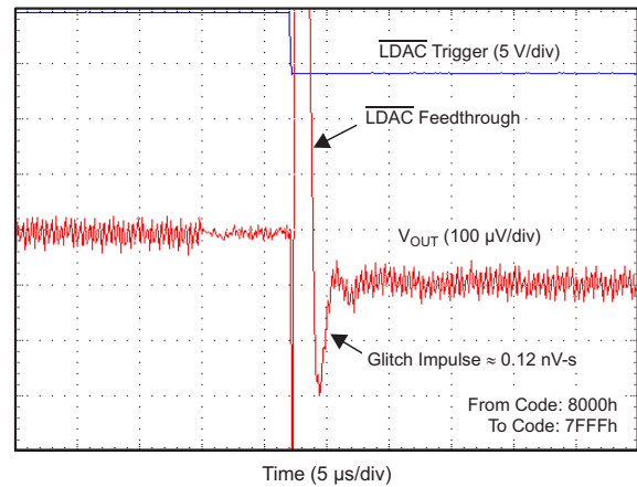
Figure 38. Glitch Impulse, Falling Edge, 1-LSB Step
