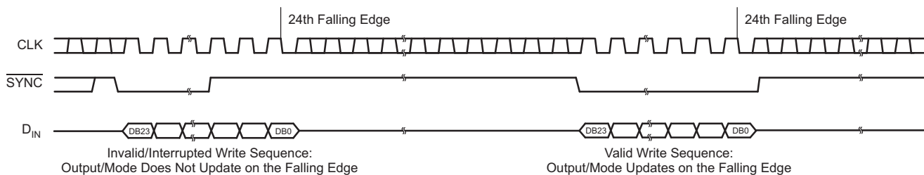
Figure 93. \overline{\text{SYNC}} Interrupt Facility
