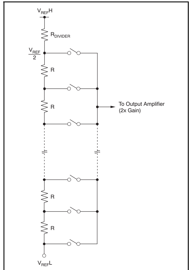
Figure 46. Resistor String
