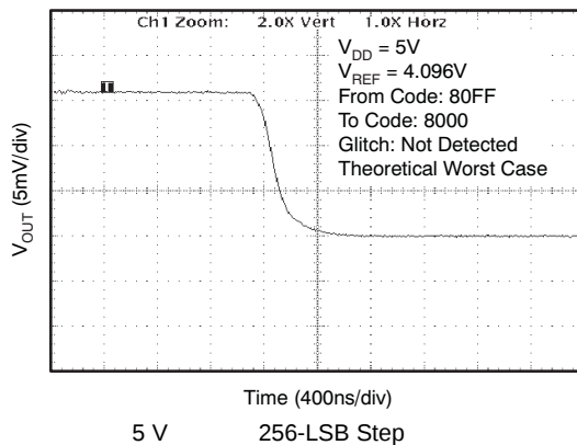
Figure 22. Glitch Energy: Falling Edge
