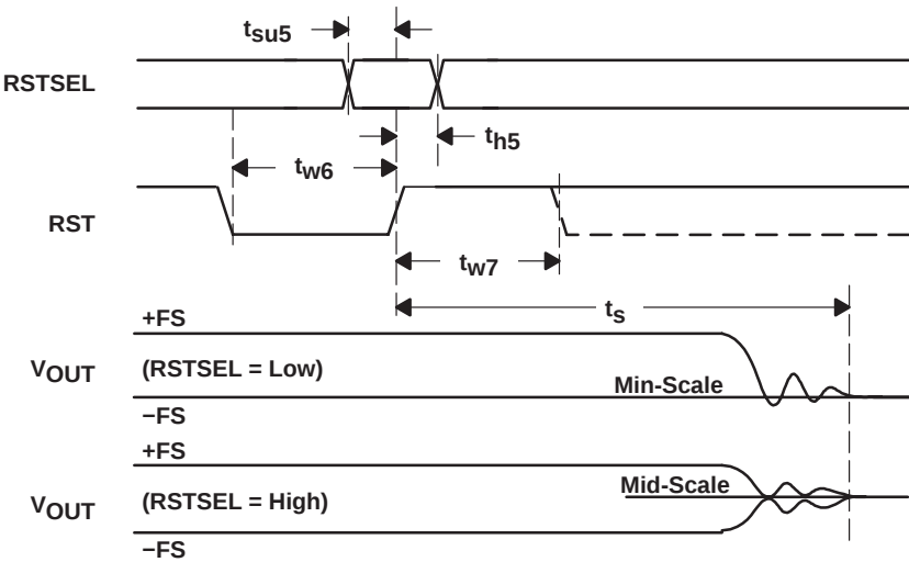
Figure 2. Reset Timing
