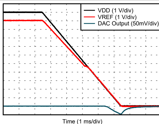
图 6-17. Full-Scale Settling Time, Falling Edge
