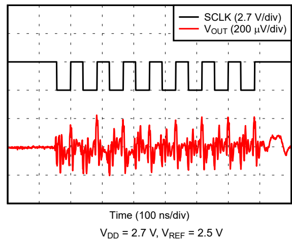
图 6-23. Clock Feedthrough
