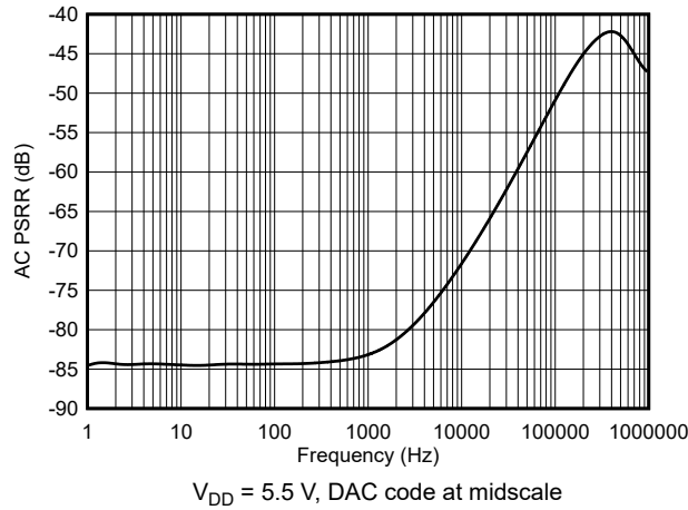
图 6-20. Power-Supply Rejection Ratio (PSRR)
