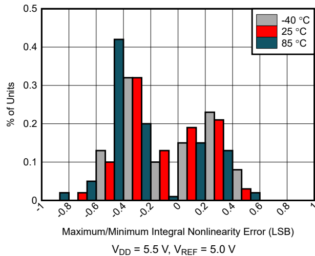
图 6-4. Integral Linearity Error Histogram
