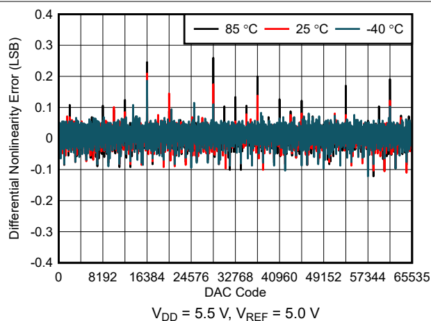
图 6-6. Differential Linearity Error vs Digital Input Code
