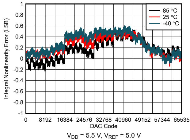
图 6-2. Integral Linearity Error vs Digital Input Code
