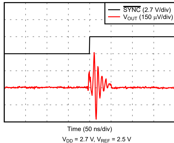
图 6-24. Control Feedthrough
