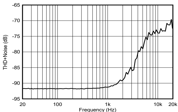
图 8-2. THD+N vs Frequency
