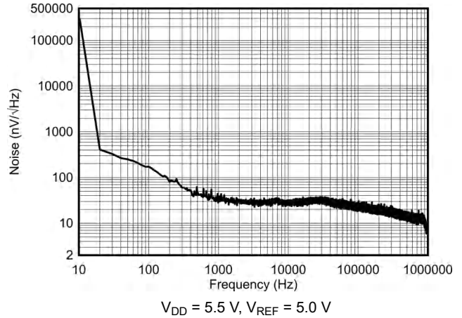
图 6-21. Output Noise Density vs Frequency
