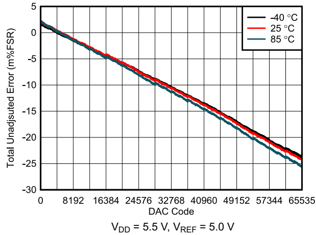
图 6-8. Total Unadjusted Error vs Digital Input Code
