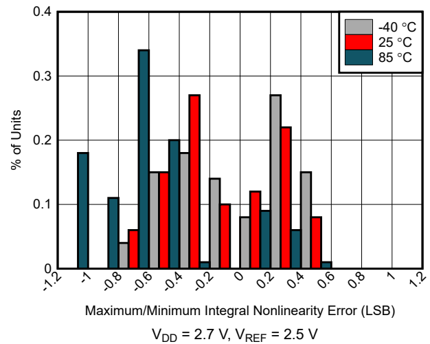
图 6-5. Integrated Linearity Error Histogram
